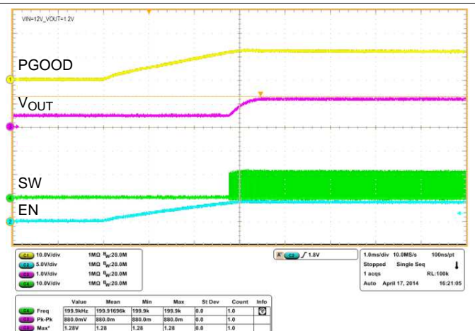
图 64. Pre-Bias Start-Up
