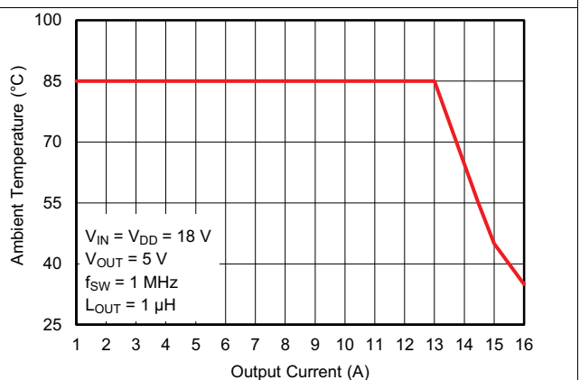
图 12. Safe Operating Area, V_{OUT} = 5\text{ V}
