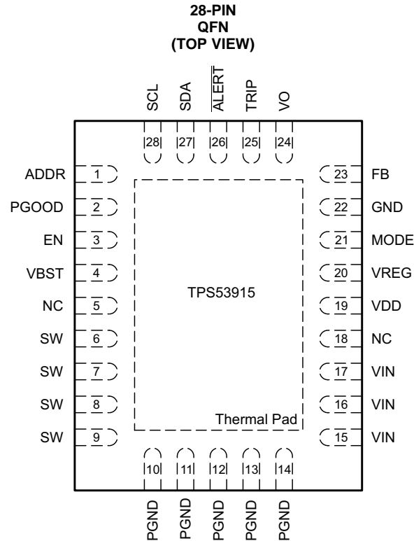
Pin Functions (1)
