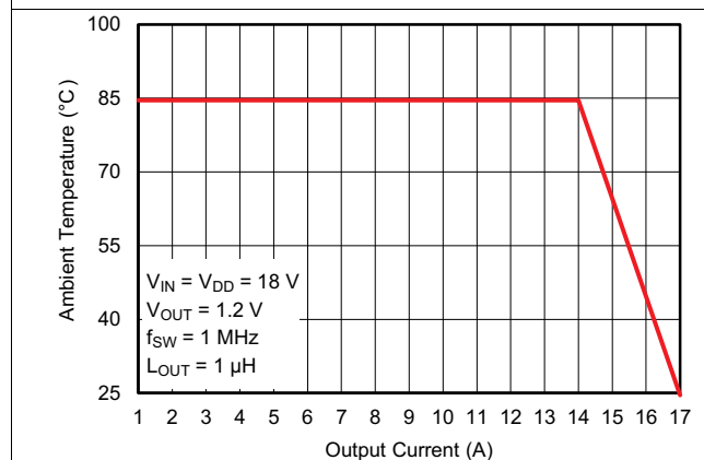
图 11. Safe Operating Area, V_{OUT} = 1.2\text{ V}
