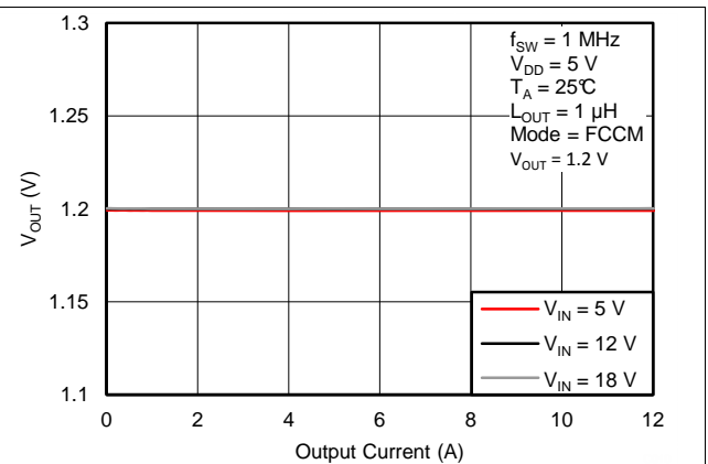
图 8. Output Voltage vs. Output Current
