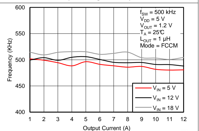
图 10. Switching Frequency vs. Output Current
