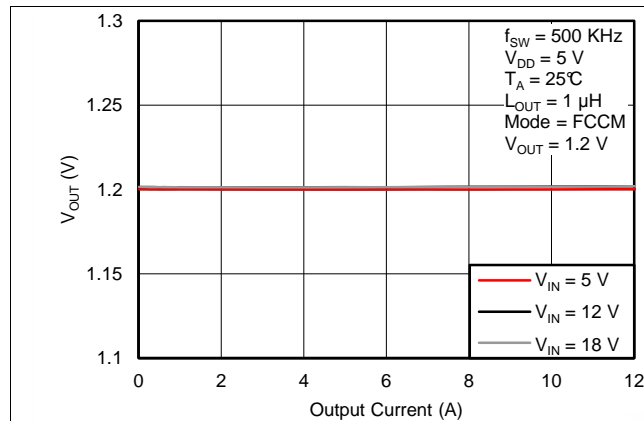
图 7. Output Voltage vs. Output Current
