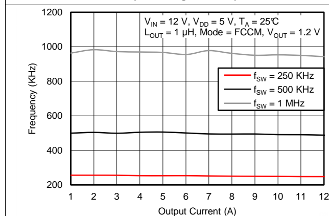
图 9. Switching Frequency vs. Output Current
