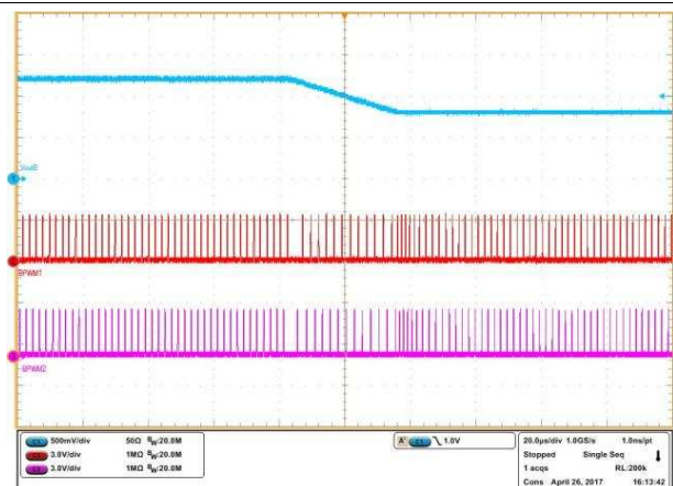
V_{VIN} = 1.2\text{ V} I_{OUT\_B} = 30\text{ A} V_{OUT\_B} VID step from 1.2 V to 0.8 V
