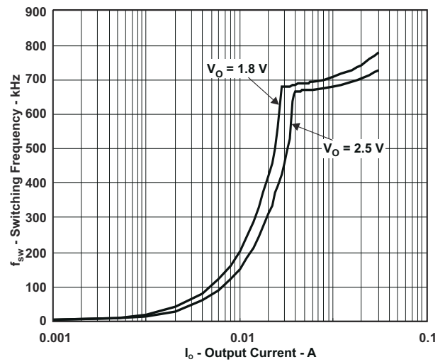
图 6-10. Switching Frequency vs Output Current
