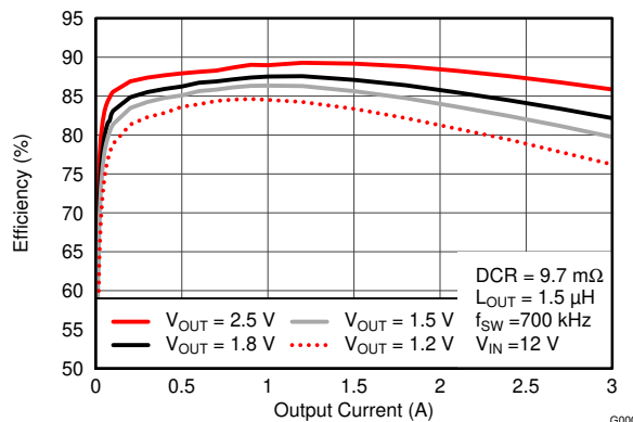
图 8-6. Efficiency vs. Output Current
