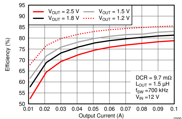
图 8-7. Light-Load Efficiency vs. Output Current
