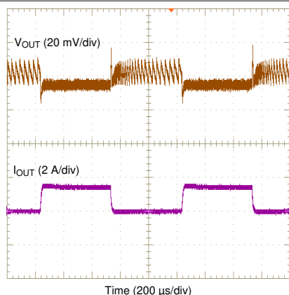
图 6-5. Load Transient Response, 1.05 V, 0 A to 1.5 A
