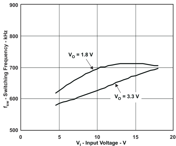
图 8-8. Switching Frequency vs. Input Voltage
