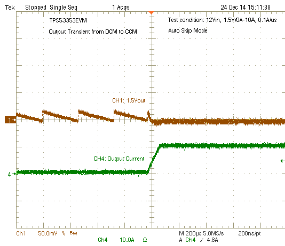
图 8-7. Output Transient from DCM to CCM
