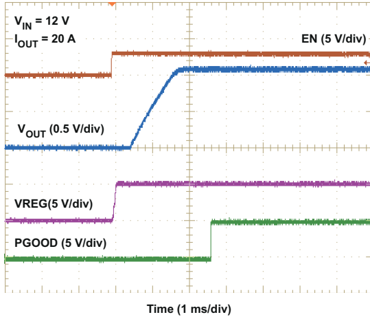
图 6-13. Start-Up Waveforms
