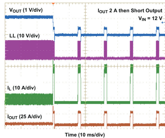
图 6-24. Output Short-Circuit Protection Waveforms
