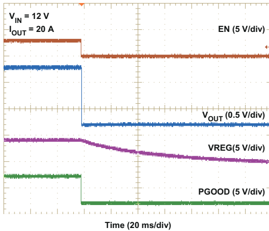
图 6-15. Shutdown Waveforms
