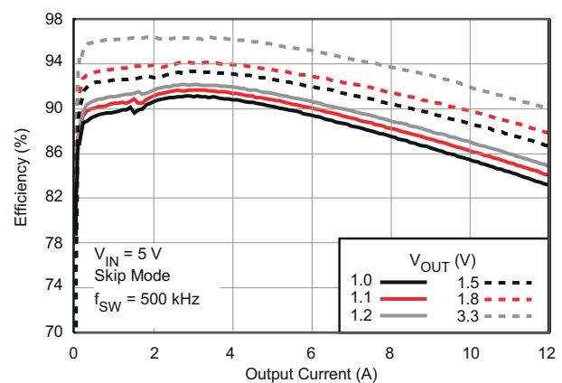
Figure 5-16. Efficiency vs Output Current
