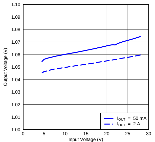
图 9. Line Regulation
