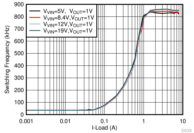
图 6-20. F_{SW} Load Regulation, OOA-mode, F_{SW} = 800 \text{ kHz}
