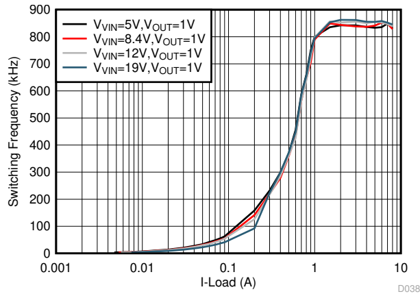
图 6-19. F_{SW} Load Regulation, Eco-mode, F_{SW} = 800 \text{ kHz}
