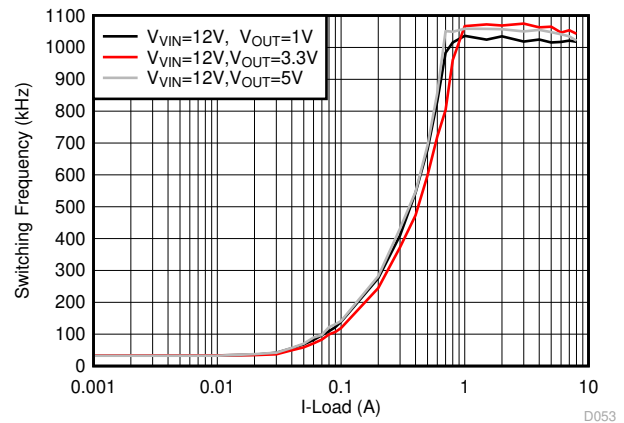
图 6-22. F_{SW} Load Regulation, OOA-mode, F_{SW} = 1 \text{ MHz}
