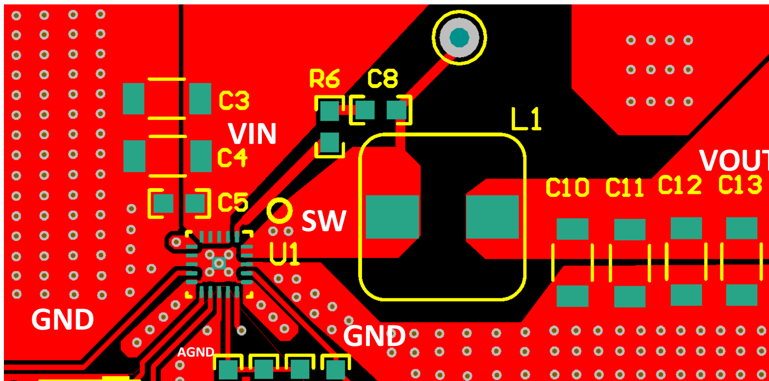
图 10-1. Top-Layer Layout
