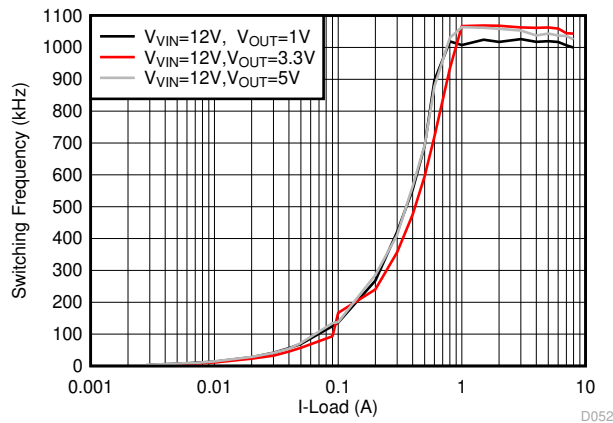
图 6-21. F_{SW} Load Regulation, Eco-mode, F_{SW} = 1 \text{ MHz}
