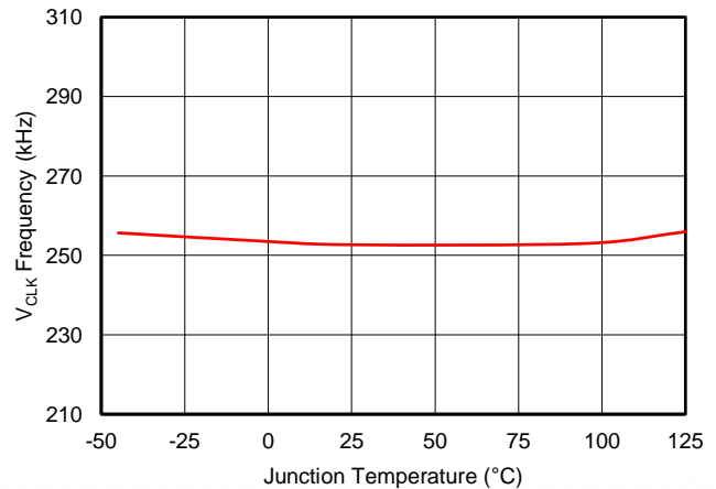
Figure 14. Clock Frequency vs. Junction Temperature
