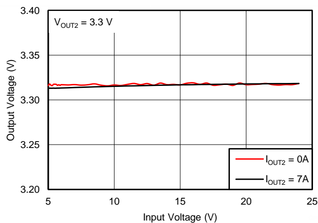
Figure 20. Line Regulation
