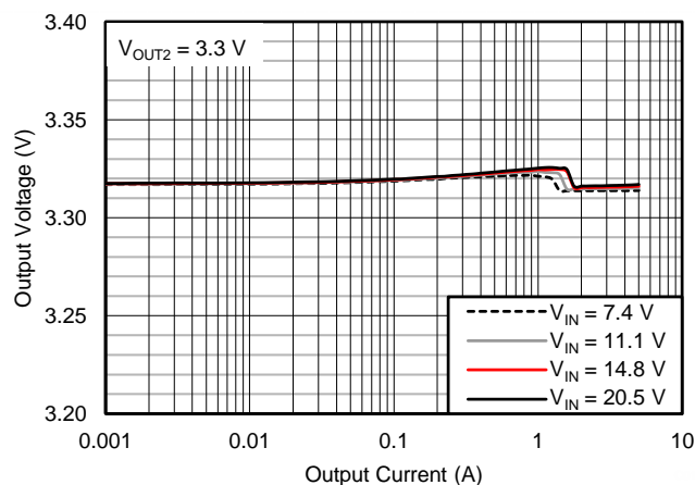
Figure 18. Load Regulation
