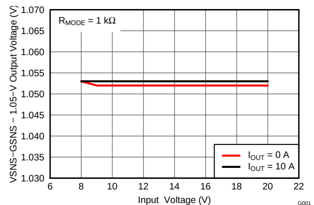
Figure 12. 1.05-V Output Line Regulation
