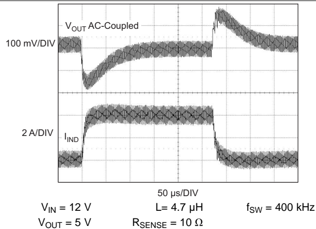
Figure 3. Buck Load Step: Forced Continuous Mode (0 to 4 A at 2.5 A/μs)
