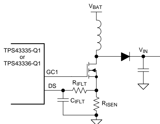
Figure 21. External Current Shunt Resistor
