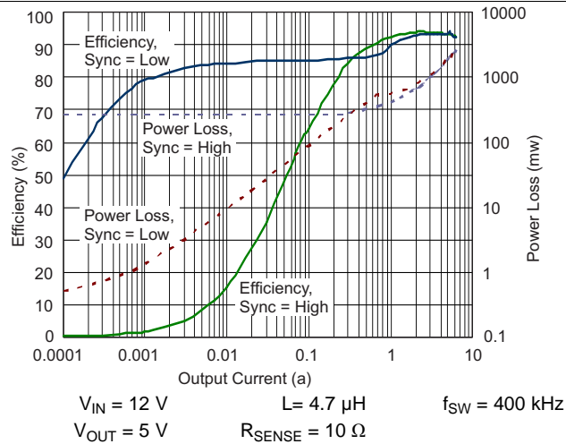
Figure 1. Efficiency Across Output Currents (Bucks)
