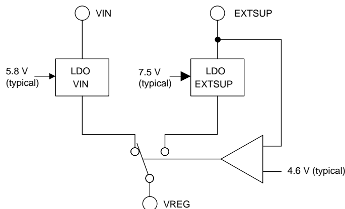
Figure 22. Internal Gate-Driver Supply
