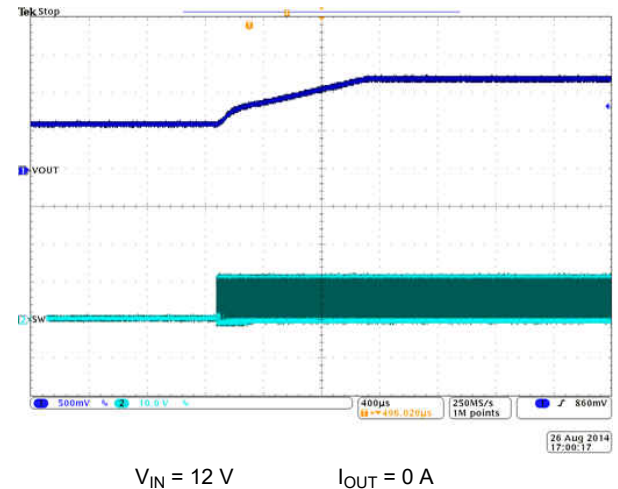
图 9-5. Prebias Start-Up
