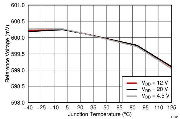
图 7-2. Reference Voltage vs. Junction Temperature
