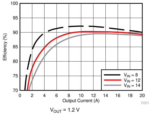
图 9-2. Efficiency vs Output Current
