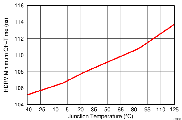
图 7-8. HDRV Minimum Off-Time vs. Junction Temperature
