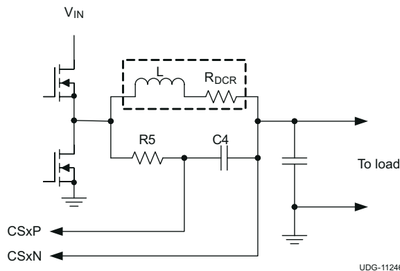
图 8-2. Current Sensing Using Inductor Resistance
