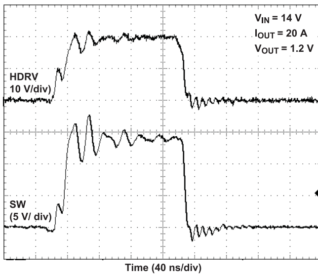
Figure 25. Switching Waveform
