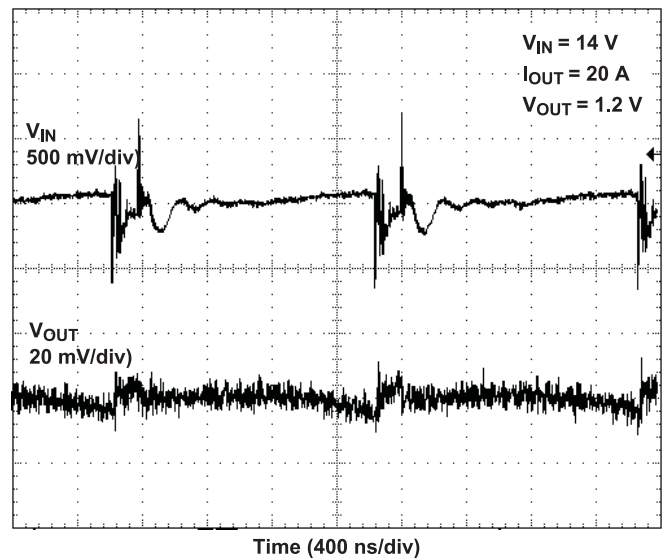
Figure 26. Ripple Waveform
