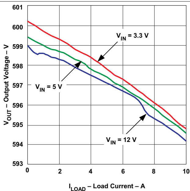
Figure 24. Line and Load Regulation
