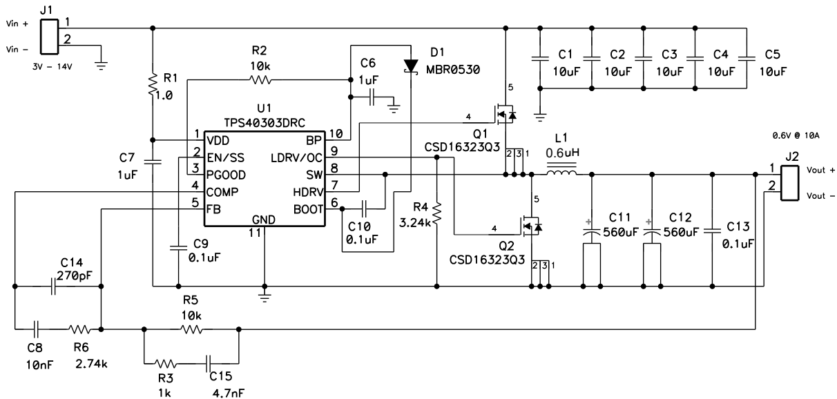
Figure 22. TPS40303 Design Example Schematic
