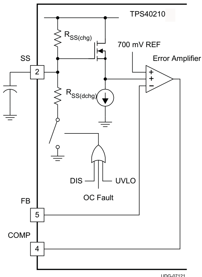
Figure 26. SS Pin Functional Circuit
