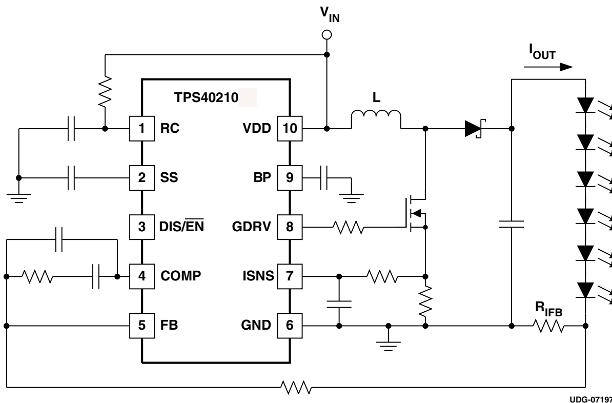
Figure 30. Typical LED Drive Schematic
