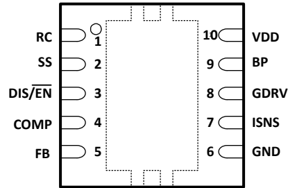
Pin Functions
