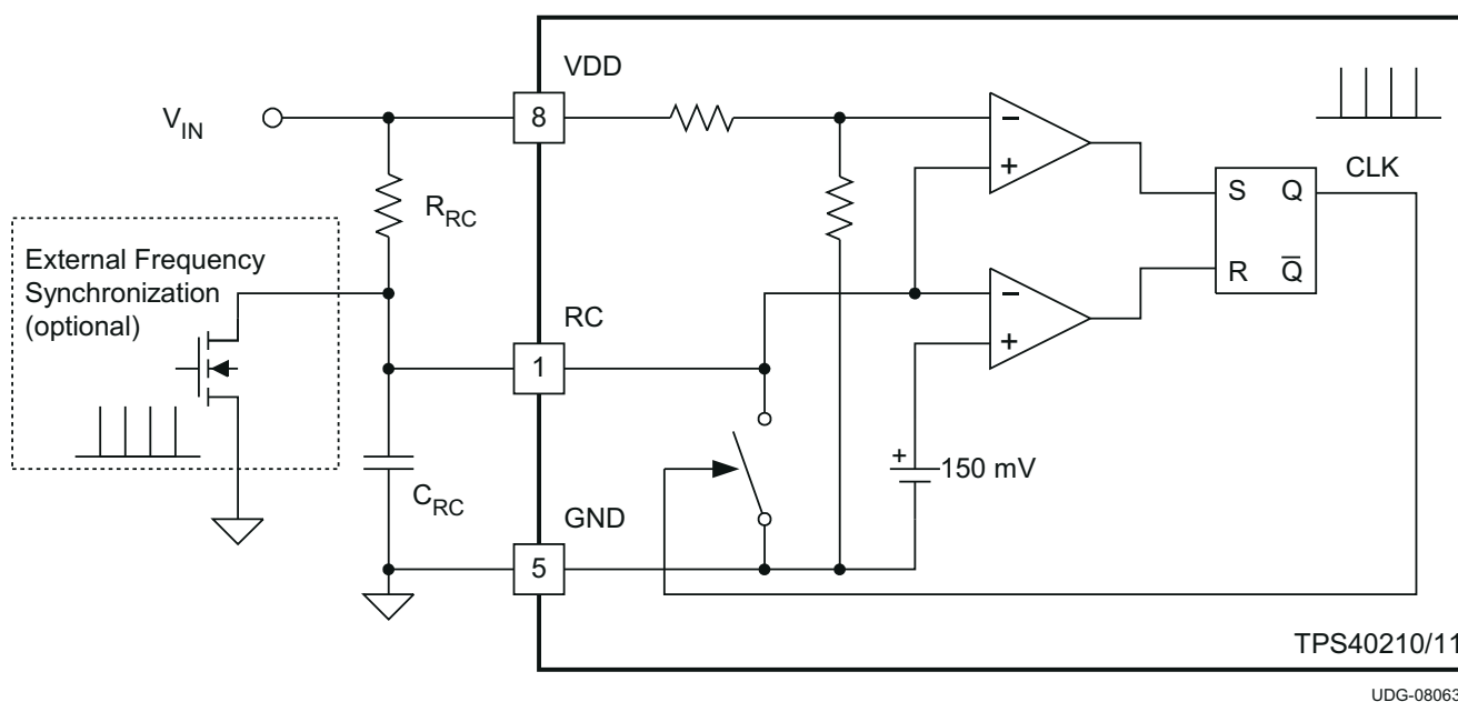
Figure 7-4. Oscillator Functional Diagram
