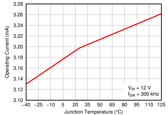
图 5-6. Operating Current vs Junction Temperature
