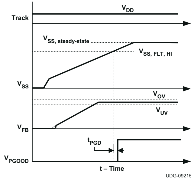
图 6-17. PGOOD Signal
