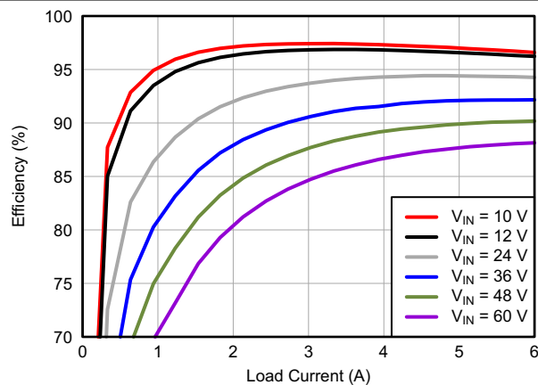
图 7-2. Efficiency vs Load Current
