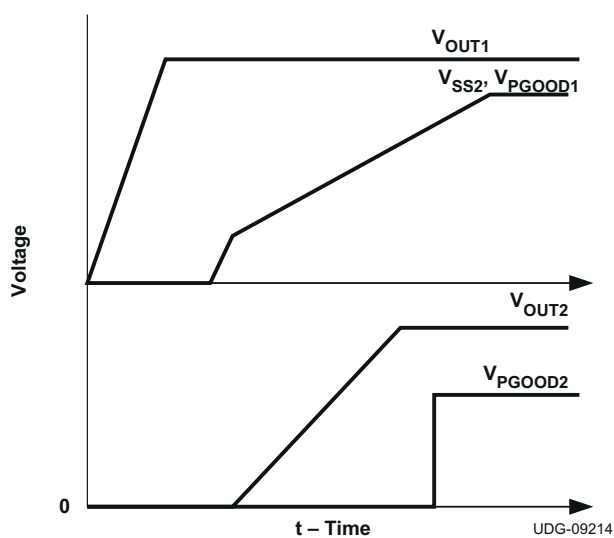
图 6-15. Sequential Start-Up Waveform
