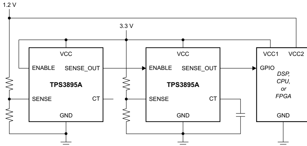
图 25. Multiple Voltage Monitoring Using ENABLE Pin
