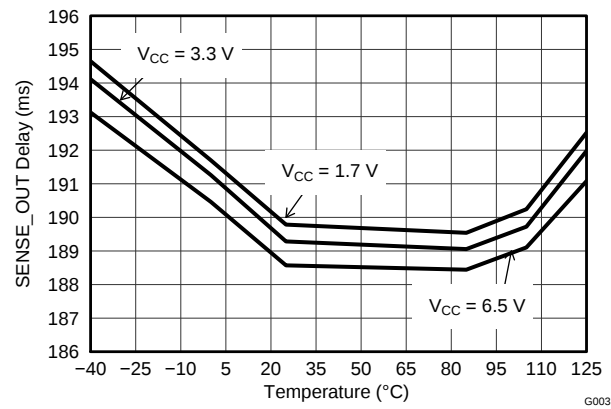
图 30. SENSE_OUT Time-out Period vs Temperature ( C_{CT} = 47 nF)
