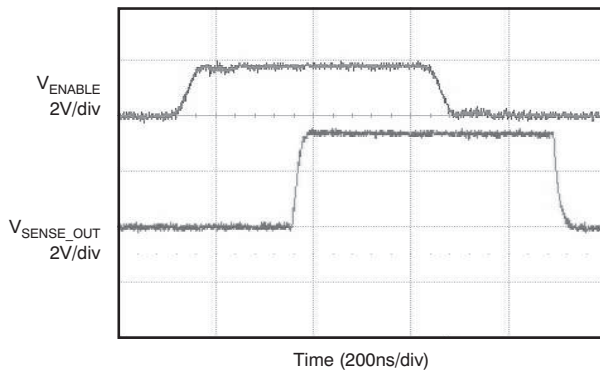
图 17. Enable Power On and Power Off Delay (TPS3895P)
