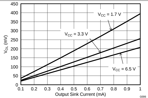
图 10. Output Voltage Low vs Output Current (0 mA to 1 mA)
