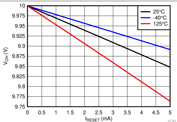
图 24. High Level Output Voltage vs I_{RESET} for TPS3840PL49
