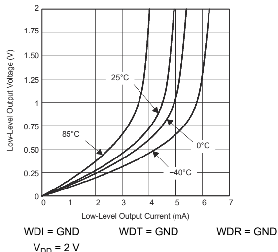
图 6-3. Low-Level Output Voltage vs Low-Level Output Current
