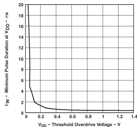
图 6-6. Minimum Pulse Duration at V_{DD} vs V_{DD} Threshold Overdrive Voltage
