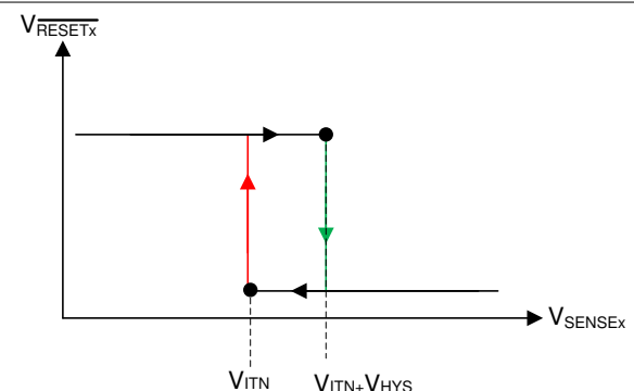
图 8-6. Hysteresis (Undervoltage Active-High)
