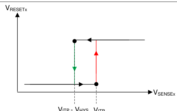
图 8-5. Hysteresis (Overvoltage Active-High)
