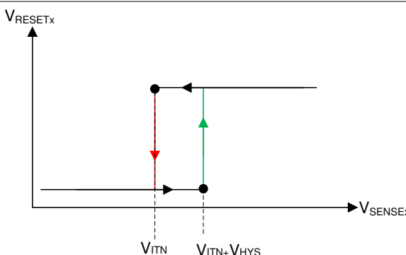
图 8-7. Hysteresis (Undervoltage Active-Low)
