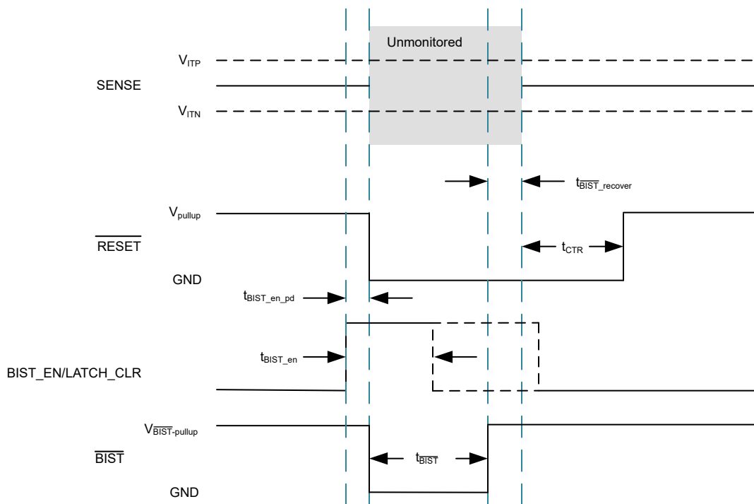
图 10-11. \overline{BIST} With \overline{RESET} Assertion
