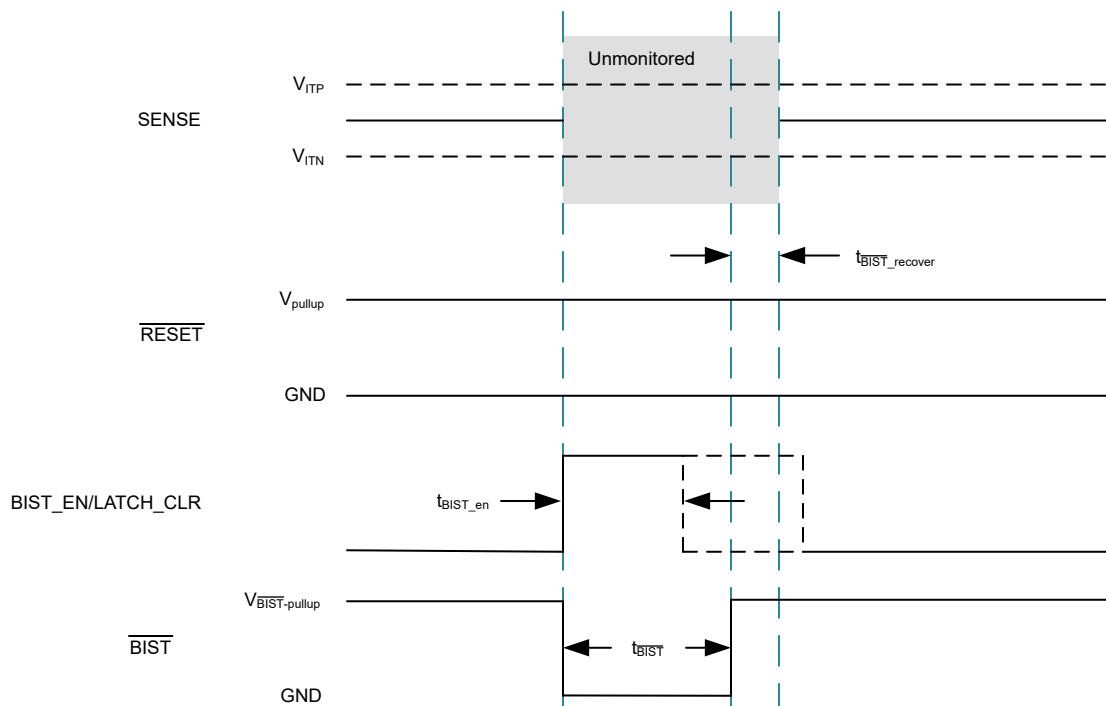
图 10-12. \overline{BIST} With No \overline{RESET} Assertion
