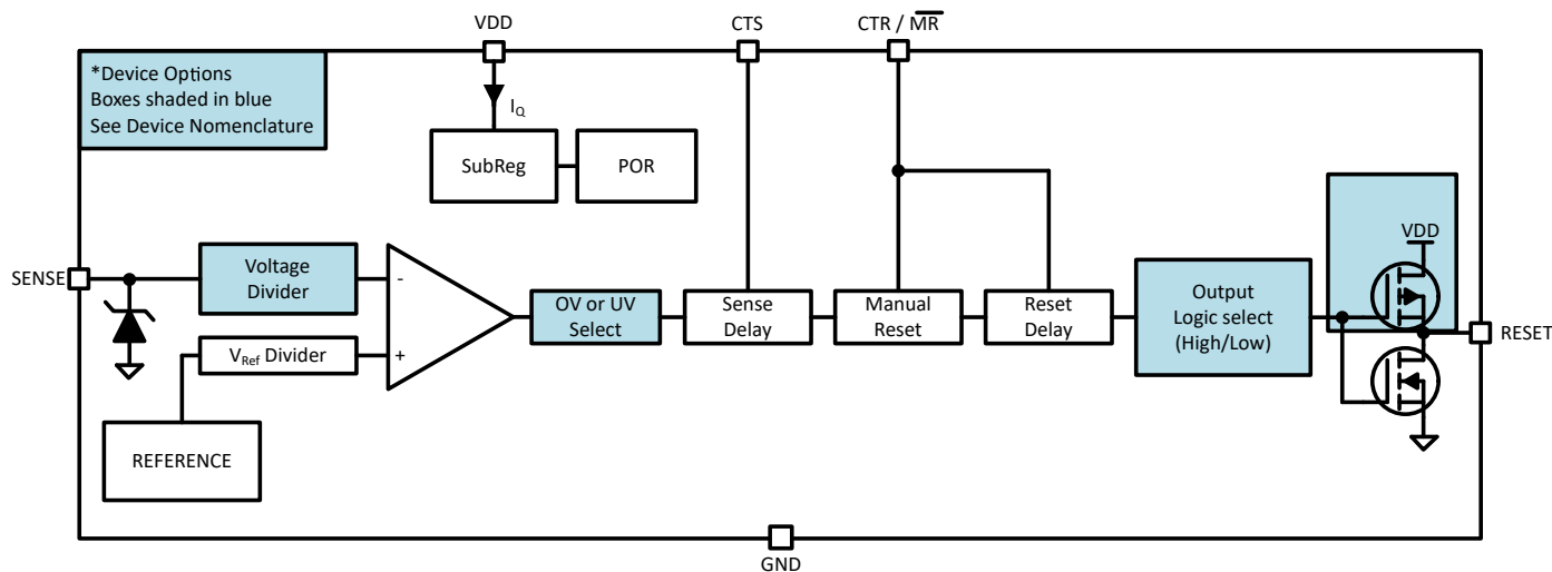
图 8-1. Functional Block Diagram 1
