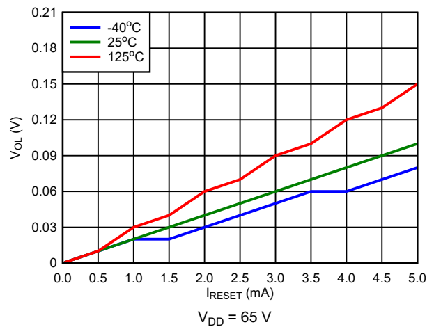
图 7-15. Open-Drain Active High V_{OL} vs I_{RESET}
