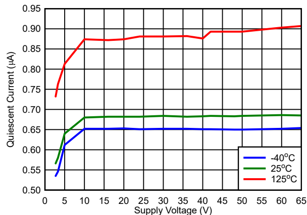
图 7-6. V_{DD} vs I_{DD} (RESET = High, V_{IT} = 2.7\text{ V} )
