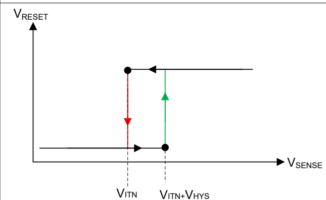
图 8-7. Hysteresis (Undervoltage Active-Low)
