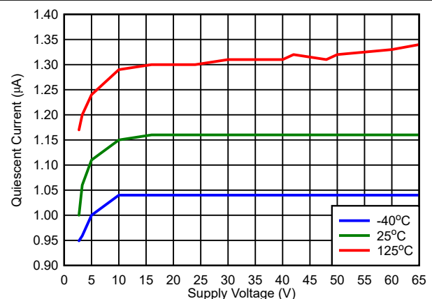
图 7-9. V_{DD} vs I_{DD} (RESET = Low, V_{IT} = 0.8\text{ V} )
