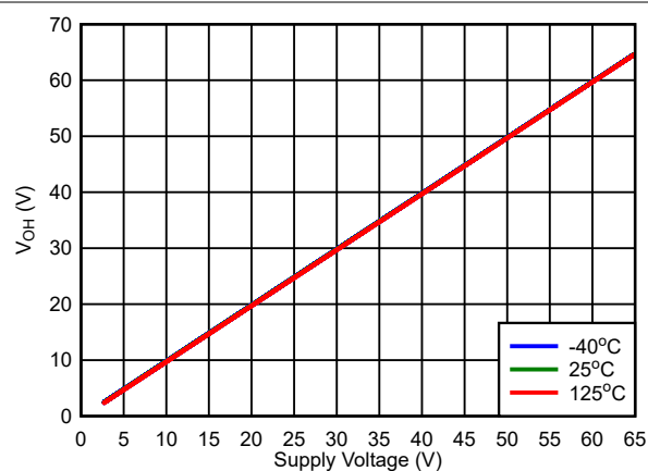
图 7-22. Push-Pull Active Low V_{OH} vs V_{DD}
