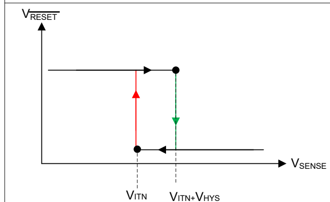
图 8-6. Hysteresis (Undervoltage Active-High)
