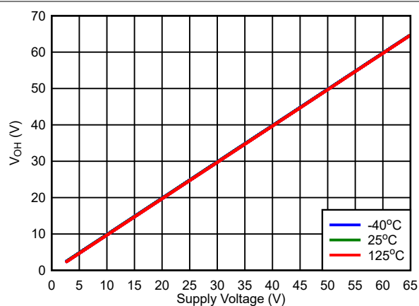
图 7-23. Push-Pull Active High V_{OH} vs V_{DD}
