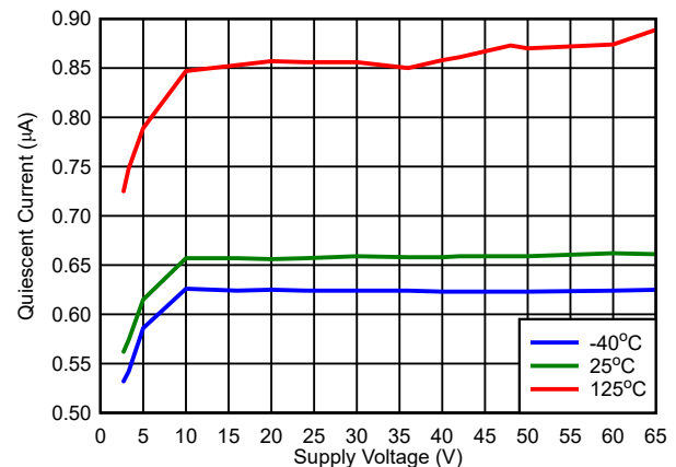
图 7-7. V_{DD} vs I_{DD} (RESET = Low, V_{IT} = 2.7\text{ V} )
