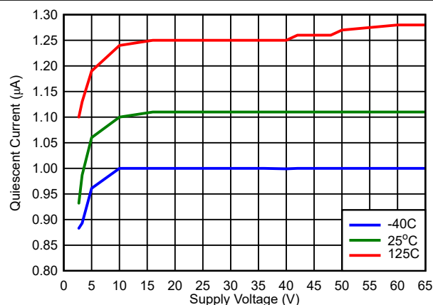
图 7-8. V_{DD} vs I_{DD} (RESET = High, V_{IT} = 0.8\text{ V} )
