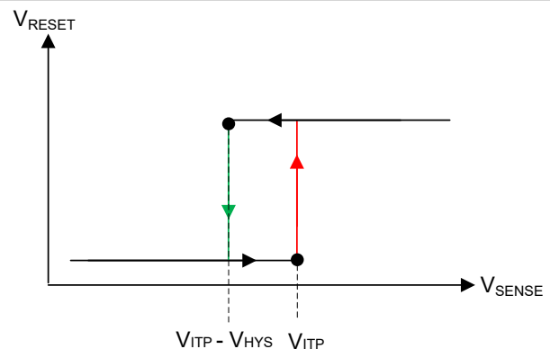
图 8-5. Hysteresis (Overvoltage Active-High)
