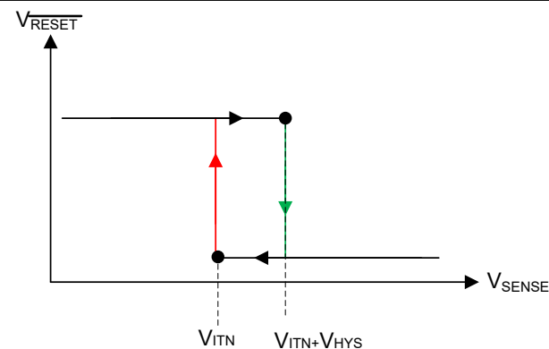
图 8-6. Hysteresis (Undervoltage Active-High)
