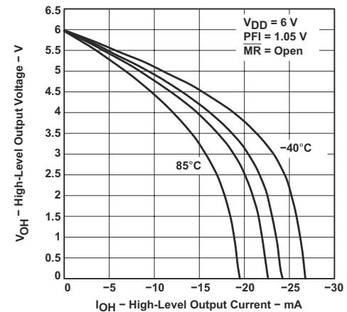
图 7-7. High-Level Output Voltage vs High-Level Output Current
