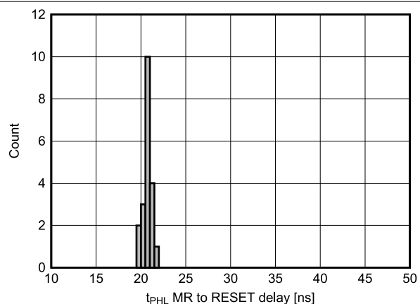
图 7-16. \overline{\text{MR}} to \overline{\text{RESET}} ( t_{\text{PHL}} ) Delay Histogram for TPS3705-33 Devices at 25°C (Unit Count = 20)
