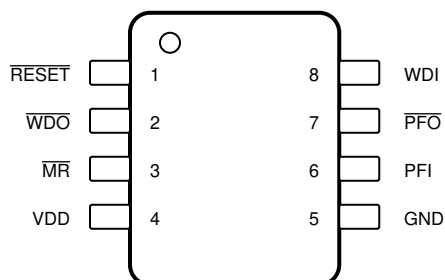
图 6-3. TPS3705-xx DGN Package 8-Pin MSOP-PowerPAD Top View
