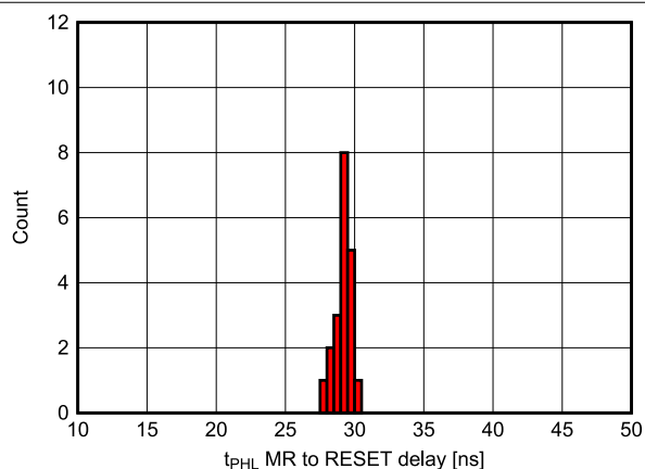
图 7-17. \overline{\text{MR}} to \overline{\text{RESET}} ( t_{\text{PHL}} ) Delay Histogram for TPS3705-33 Devices at 125°C (Unit Count = 20)
