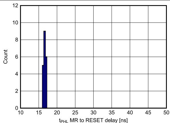
图 7-15. \overline{\text{MR}} to \overline{\text{RESET}} ( t_{\text{PHL}} ) Delay Histogram for TPS3705-33 Devices at -40°C (Unit Count = 20)
