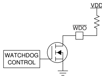
图 8-7. Open-Drain \overline{\text{WDO}} Configuration
