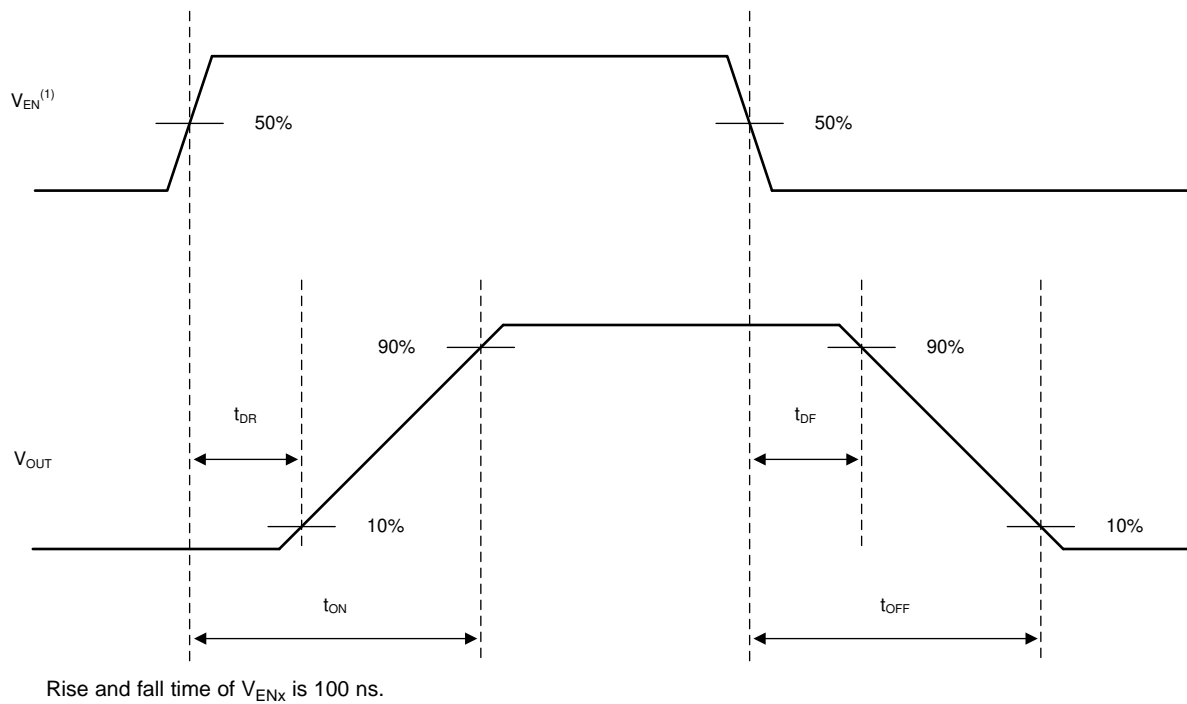
图 1. Switching Characteristics Definitions
