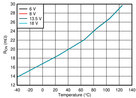
图 9. On Resistance ( R_{ON} ) vs Temperature
