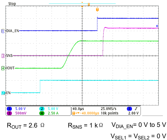
图 7-29. I_{SNS} Settling Time ( t_{SNSION1} ) on DIA_EN Transition
