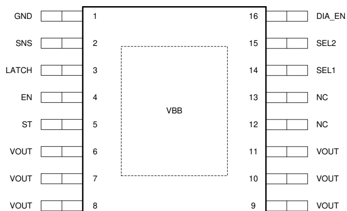
图 6-1. PWP Package 16-Pin HTSSOP Top View
