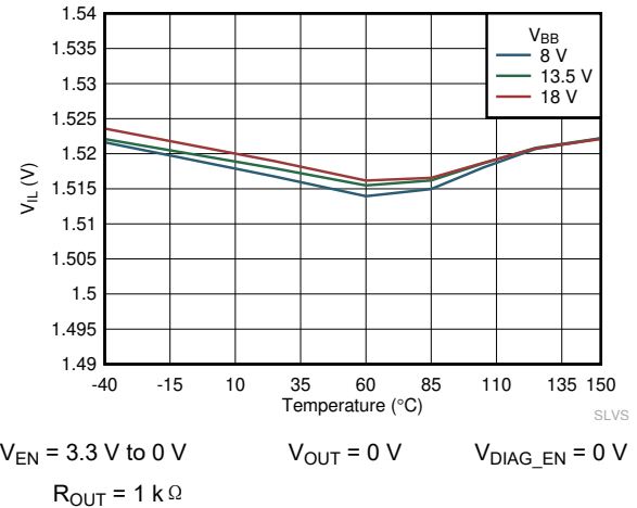
图 7-22. V_{IL} vs Temperature
