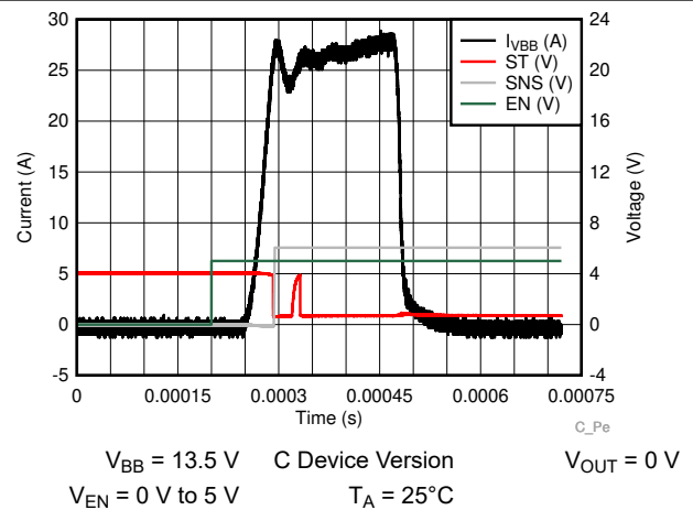
图 7-32. Short Circuit Behavior
