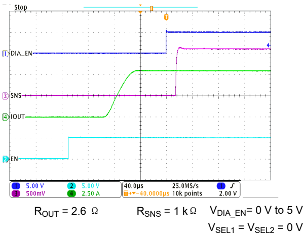
图 7-29. I_{SNS} Settling Time ( t_{SNSION1} ) on DIA_EN Transition
