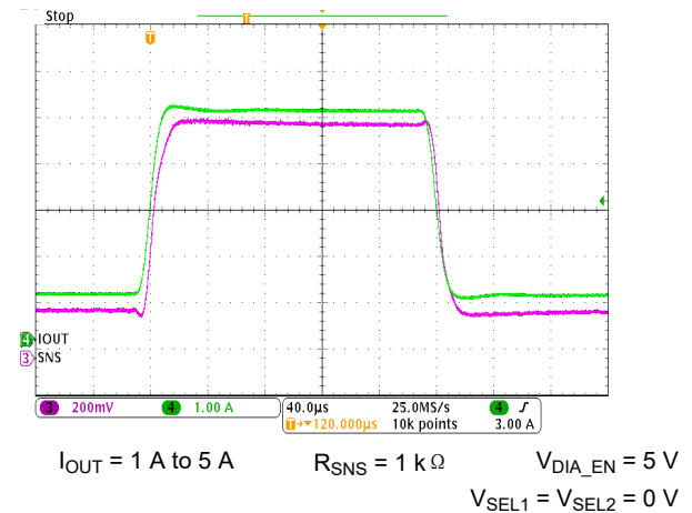
图 7-30. I_{SNS} Settling Time ( t_{SETTLEH} ) on Rising Load Step
