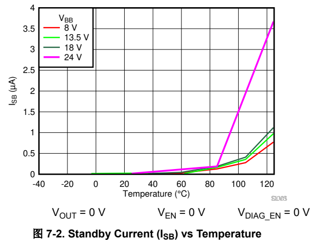
图 7-2. Standby Current ( I_{SB} ) vs Temperature
