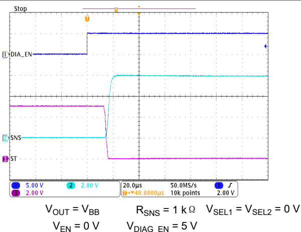
图 7-31. Open Load Detection Time ( t_{OL2} ) on Rising DIAG_EN
