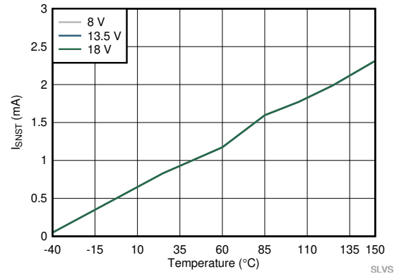
图 7-16. Temperature Sense Output Current ( I_{SNSI} ) vs Temperature
