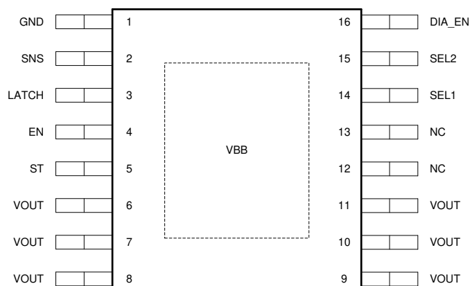
图 6-1. PWP Package 16-Pin HTSSOP Top View
