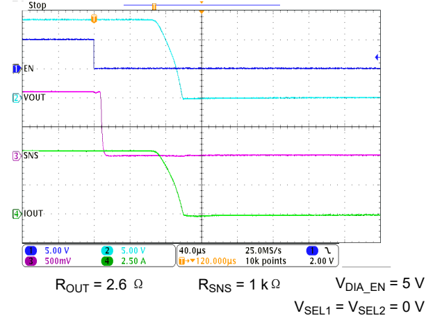
图 7-28. Turn-off Time ( t_{OFF} ) and Sense Settle Time ( t_{SNSION2} )
