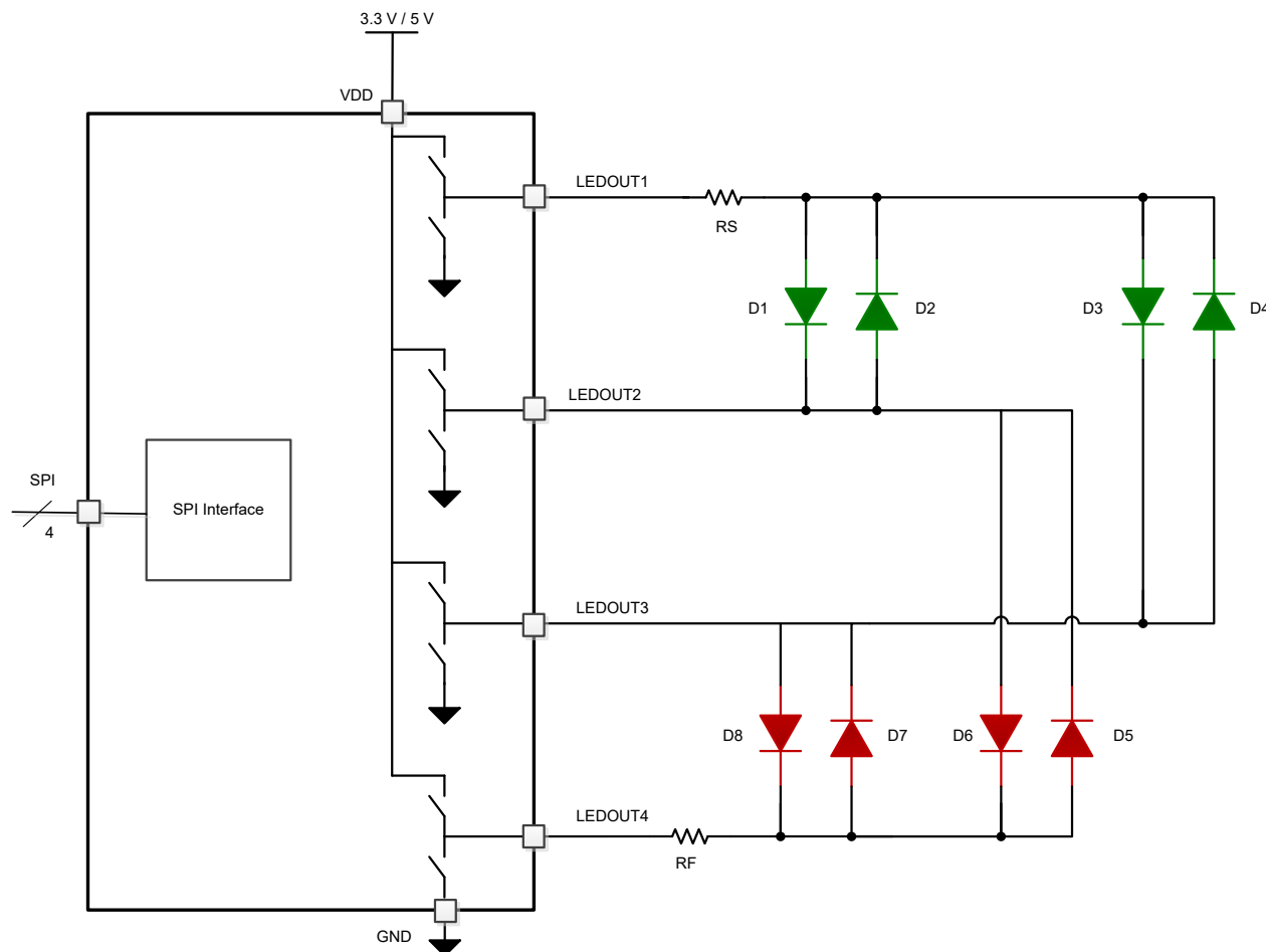
图 8-40. LED Driver
