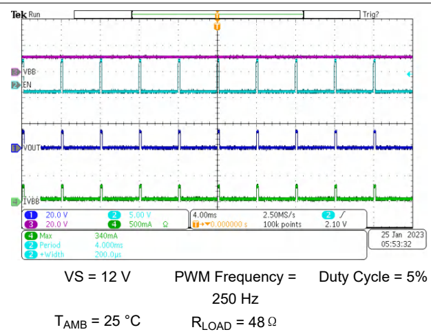
图 6-4. Switching the Part With 250-Hz PWM Signal
