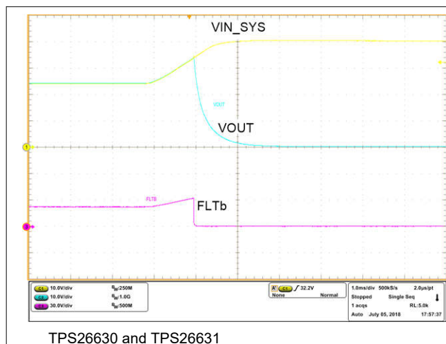
图 8-5. Overvoltage Cutoff Response at 33-V Level
