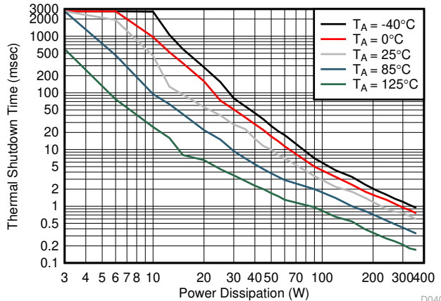
图 6-18. Thermal Shutdown Time vs Power Dissipation
