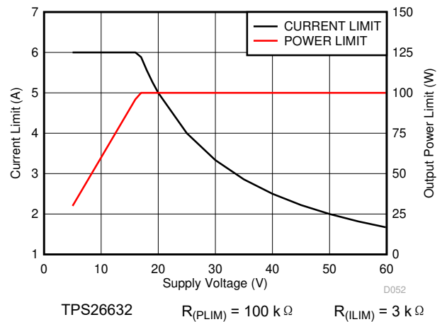
图 6-12. Power Limit, Current limit vs Supply Voltage
