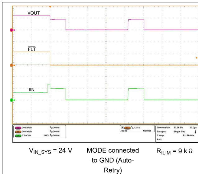
图 8-14. Overload Performance With TPS26631, TPS26633, TPS26635, and TPS6637 During Load Step from 19\ \Omega to 9\ \Omega
