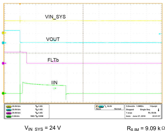
图 8-16. Output Hot-Short Response
