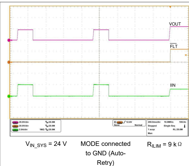
图 8-15. Response During Coming Out of Overload Fault
