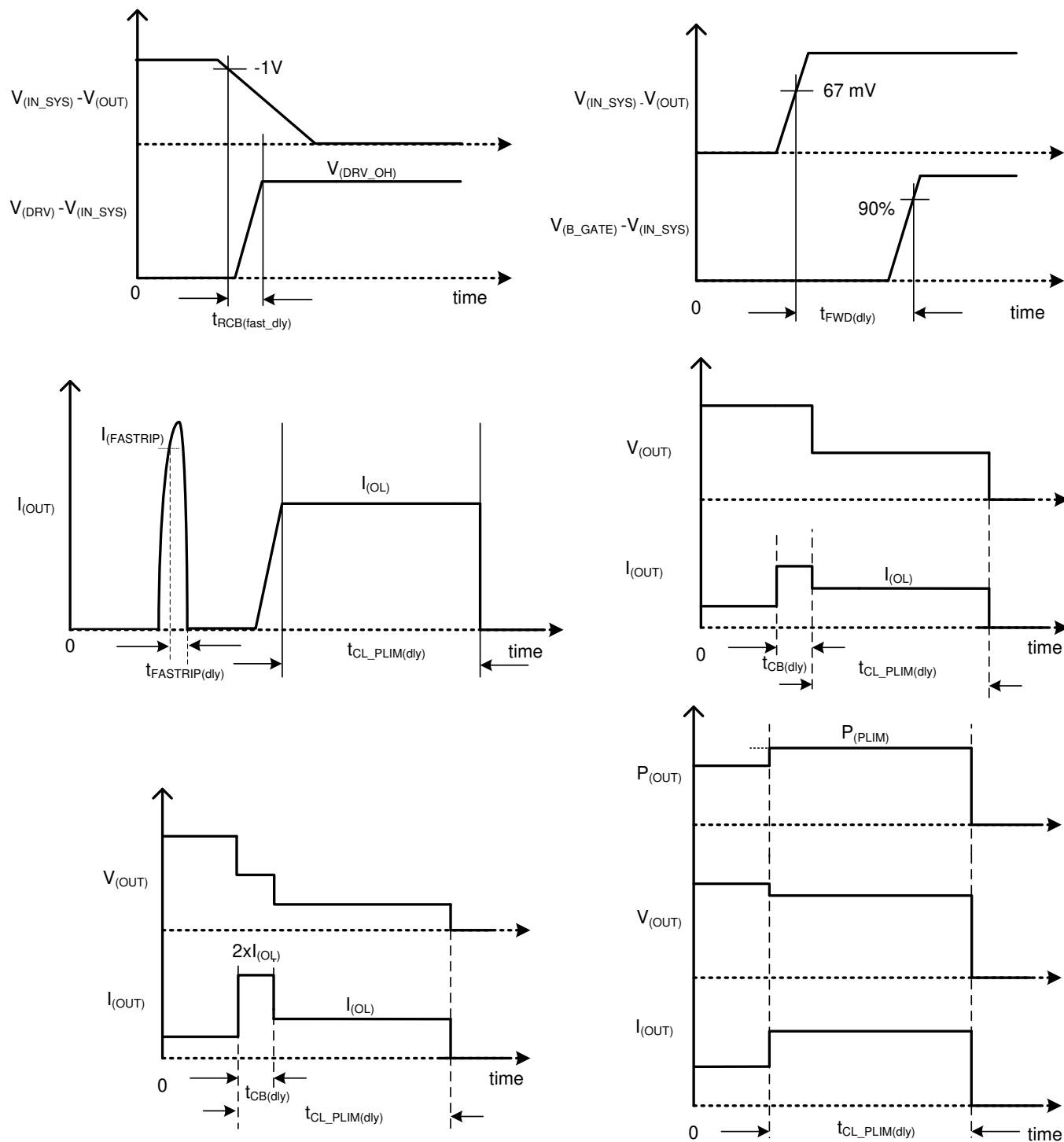
图 7-2. Timing Waveforms
