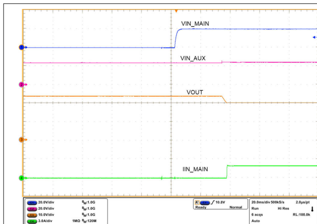
图 9-13. VIN_MAIN Power Recovery: Change Over from Auxiliary VIN_AUX to Primary Power VIN_MAIN
