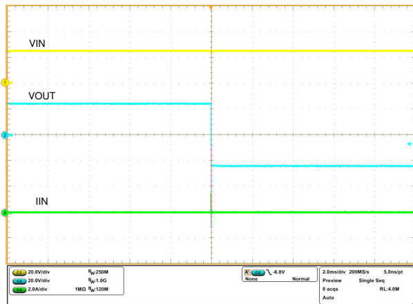
9-6. Reverse Output Polarity Protection With – 24 V at OUT and 24 V at IN
