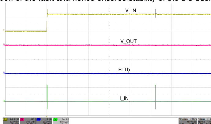
MODE pin connected to RTN VIN = 24 V R ILIM = 5.36 kΩ Figure 45. Start-Up With Short on Output
