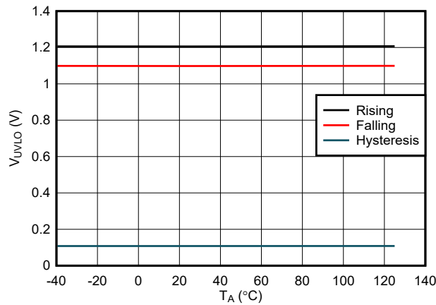
图 7-9. EN/UVLO Based Turn-off Thresholds Across Temperature
