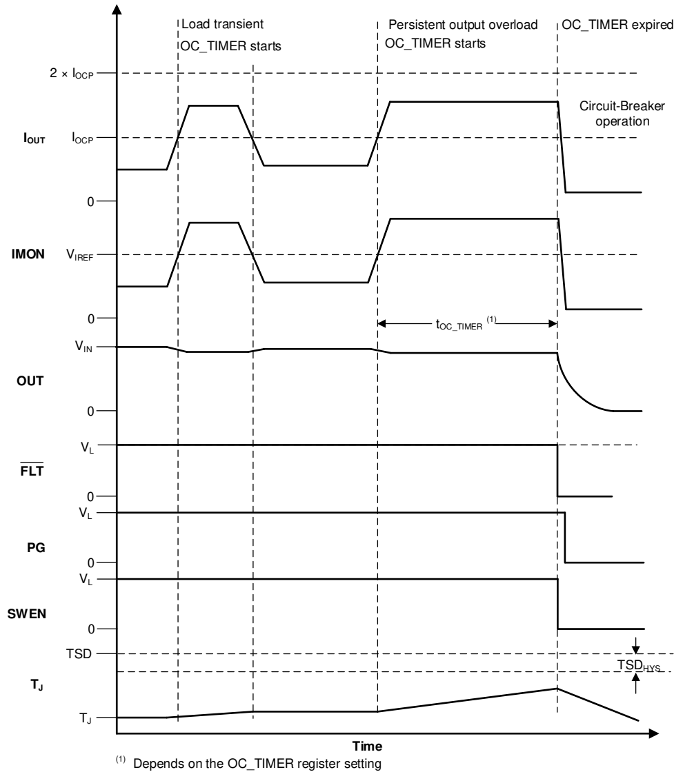
图 8-4. Steady-state Overcurrent (Circuit-Breaker) Response
