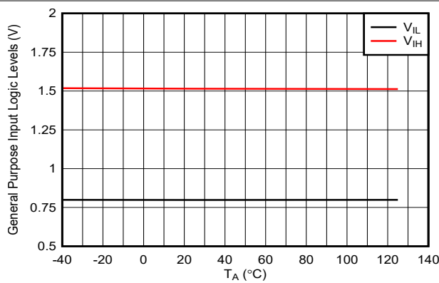
图 7-29. SWEN/General Purpose Input Pin Logic Thresholds Across Temperature
