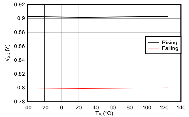
图 7-10. EN/UVLO Based Shutdown Thresholds Across Temperature
