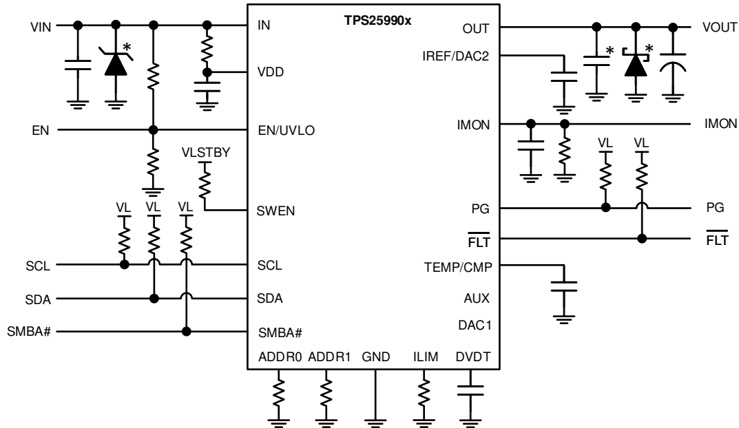
图 9-18. Circuit Implementation with Optional Protection Components
