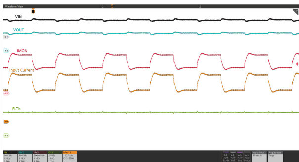
图 9-9. Transient Overload: V_{IN} = 12 V, t_{OC\_TIMER} = 10 ms, C_{LOAD} = 50 mF, R_{IMON} = 150 \Omega , V_{IREF} = 1 V, and Load Current Stepped from 333 A to 500 A then 333 A within 8.5 ms
