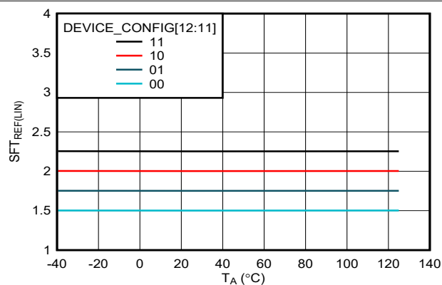
图 7-17. Scalable Fast-trip Threshold Ratio Across Temperature (Steady-state)
