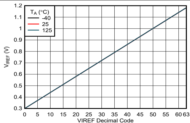
图 7-13. VIREF DAC Transfer Function
