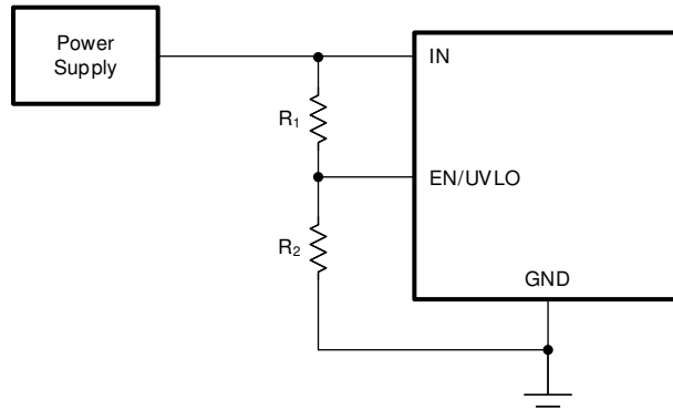
图 8-2. Adjustable Undervoltage Protection
