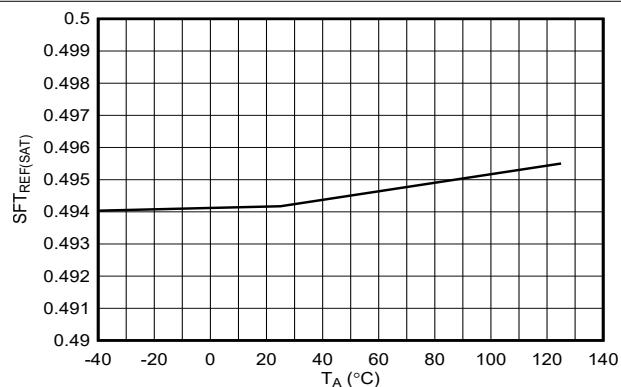
图 7-18. Scalable Fast-trip Threshold Ratio Across Temperature (Startup)
