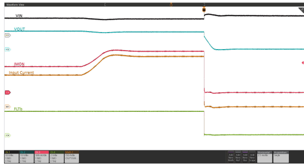
图 9-11. Circuit-Breaker Response: V_{IN} = 12\text{ V} , t_{OC\_TIMER} = 10\text{ ms} , C_{LOAD} = 50\text{ mF} , R_{IMON} = 150\ \Omega , V_{IREF} = 1\text{ V} , and Load Current Stepped from 333 A to 530 A for more than 10 ms
