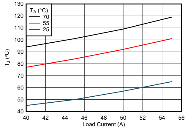
图 7-32. Junction Temperature vs Load Current (No Air-Flow)
