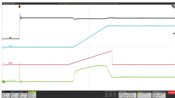
图 9-5. Input Hot Plug: V_{IN} Stepped Up from 0 V to 12 V, C_{LOAD} = 50 mF, R_{LOAD(Start-up)} = 0.48 \Omega , C_{DVRT} = 33 nF, V_{IREF} = 1 V, R_{ILIM(TPS25990)} = 422 \Omega , and R_{ILIM(TPS25985)} = 316 \Omega
