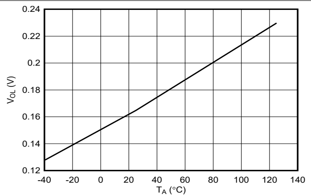
图 7-30. PGOOD/FLT/General Purpose Output Pin Logic Level Across Temperature
