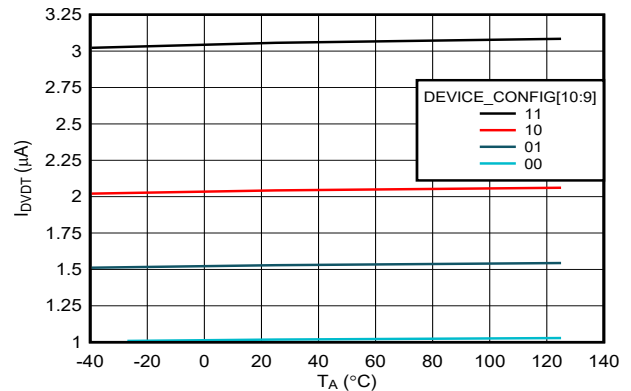
图 7-22. DVDT Pin Charging Current Across Temperature
