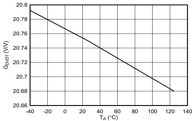
图 7-23. DVDT Gain Across Temperature
