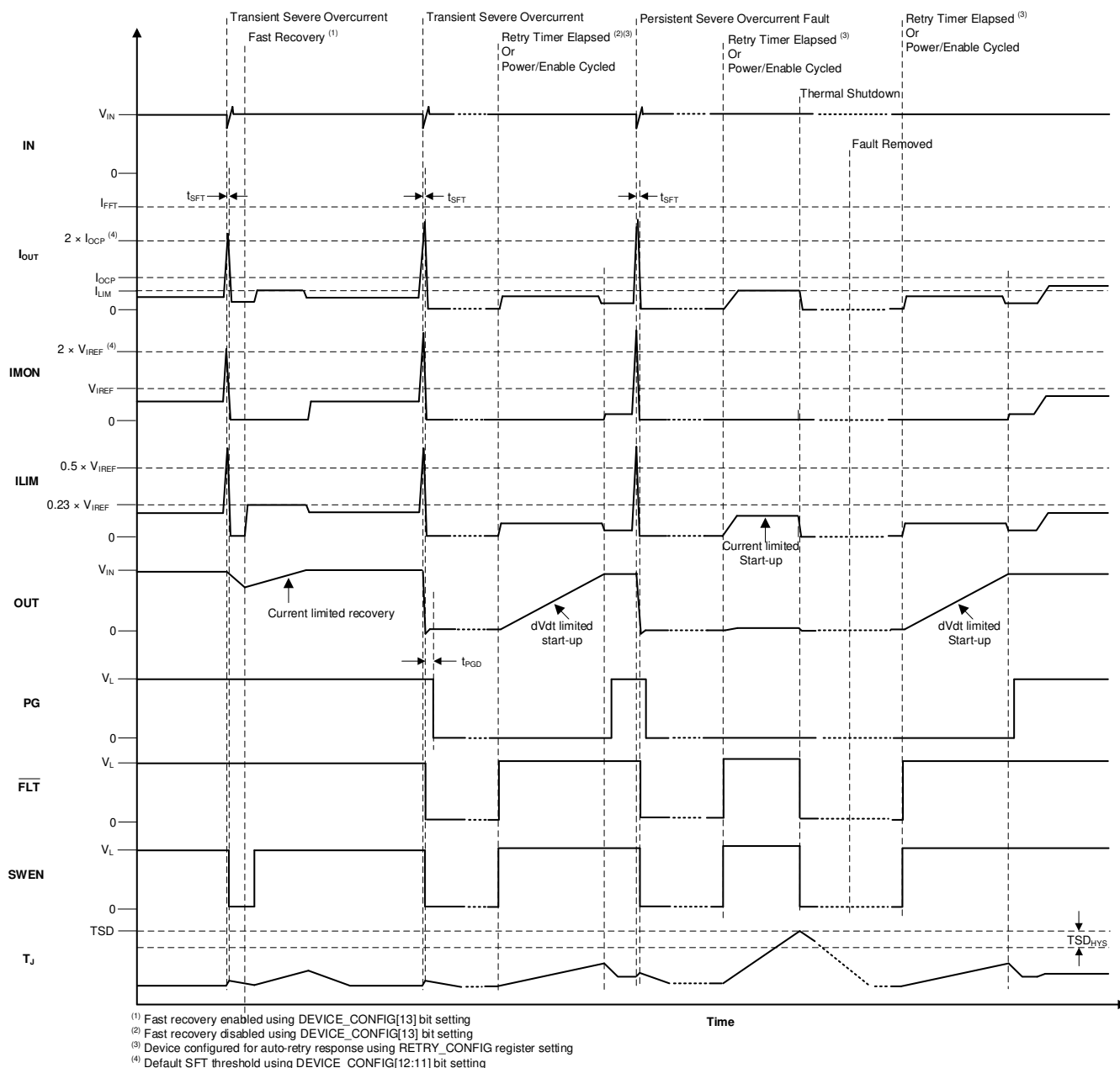
图 8-5. Short-Circuit Response
