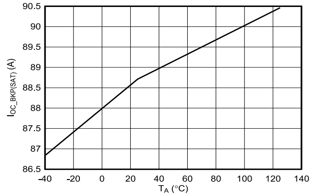
图 7-20. Backup Overcurrent Protection Threshold (Startup) Accuracy
