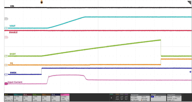
图 7-38. Power Up Using PMBus Command
