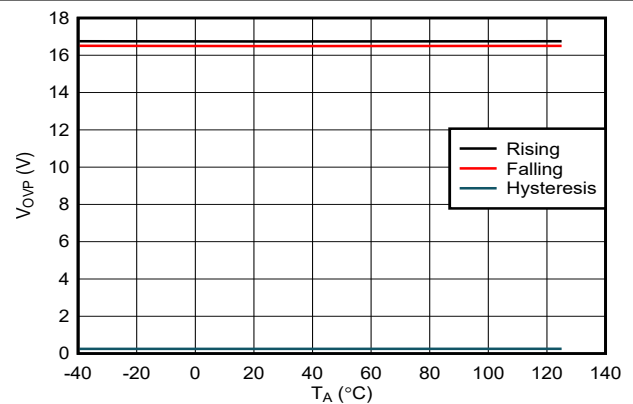
图 7-6. VIN Overvoltage Protection Threshold Across Temperature (VIN_OV_FLT = 0x0E (Default))
