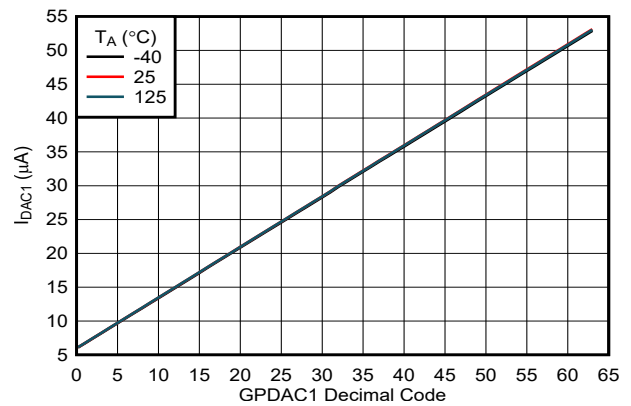
图 7-26. General Purpose DAC1 Transfer Function
