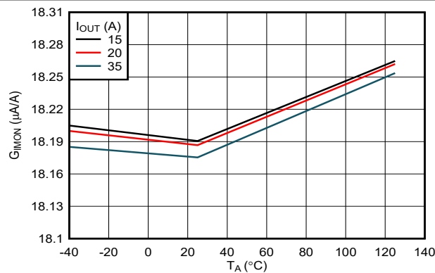
图 7-11. IMON Gain Across Load and Temperature
