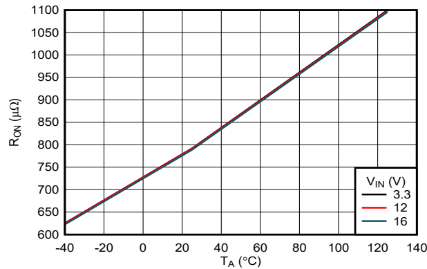
图 7-1. ON Resistance Across Temperature
