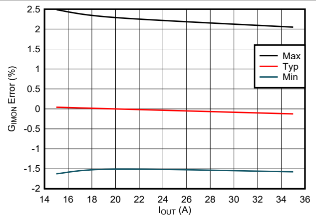
图 7-12. IMON Gain Accuracy Across Process, Voltage and Temperature Corners
