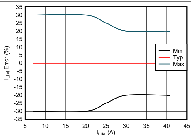
图 7-16. Startup Overcurrent Protection Threshold (Current Limit) Accuracy
