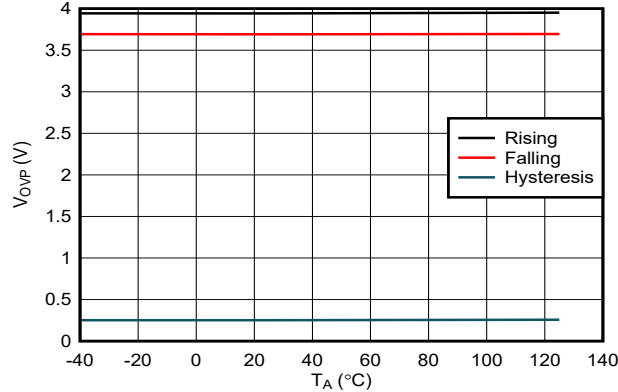
图 7-7. VIN Overvoltage Protection Threshold Across Temperature (VIN_OV_FLT = 0x01)
