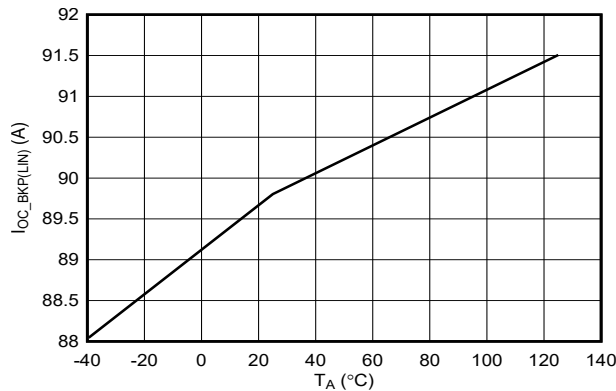
图 7-21. Backup Overcurrent Protection Threshold (Steady-state) Accuracy
