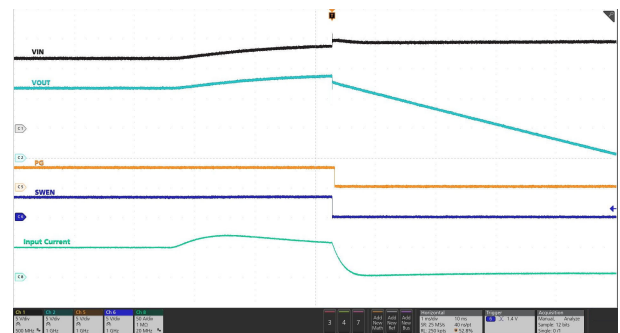
图 7-44. Input Undervoltage Protection
