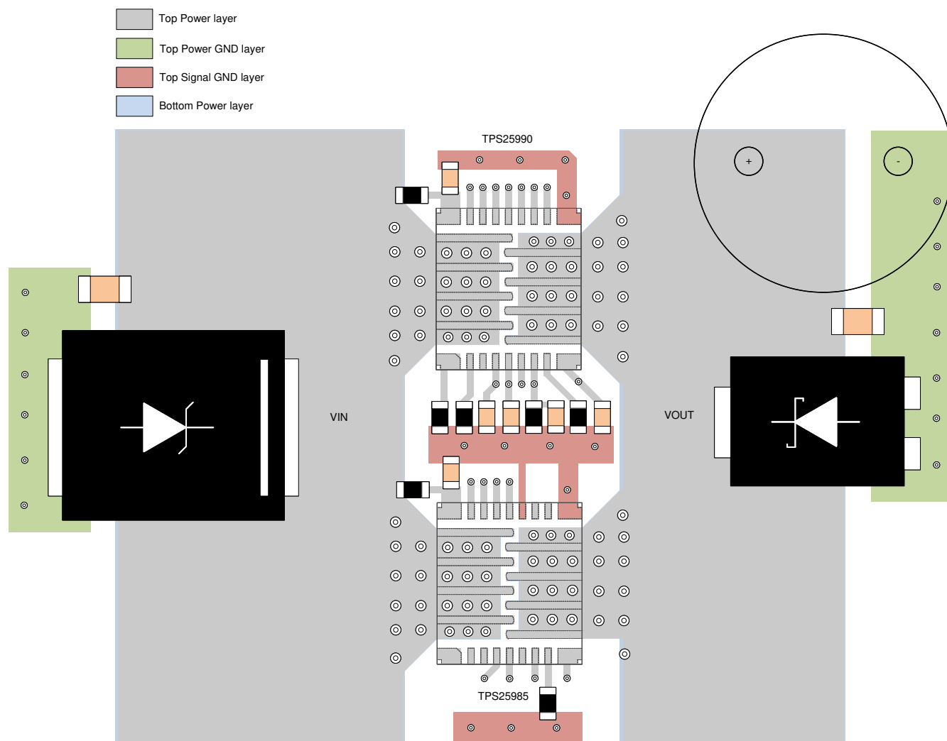
图 9-19. TPS25990 and TPS25985x Parallel Devices Layout Example
