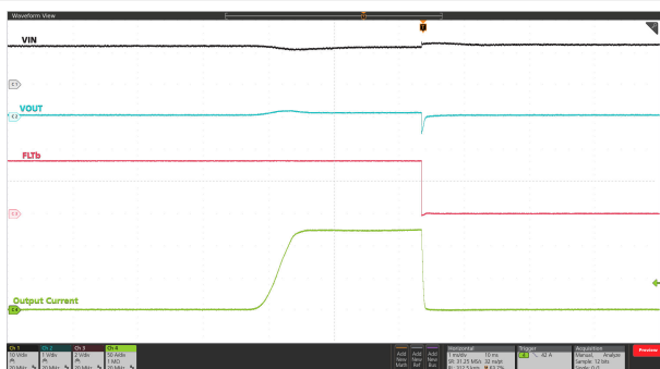
图 9-7. Power Up into Short: V_{IN} = 12 V, EN/UVLO Stepped Up From 0 V to 3 V, V_{IREF} = 1 V, R_{ILIM(TPS25990)} = 422 \Omega , R_{ILIM(TPS25985)} = 316 \Omega , and OUT Shorted to GND
