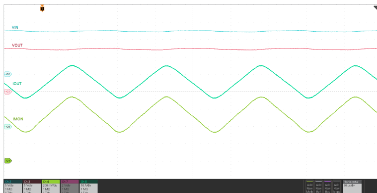
图 8-6. Analog Load Current Monitor Response
