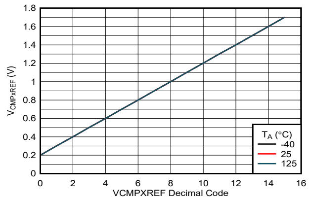
图 7-28. General Purpose Comparators Reference DAC Transfer Function
