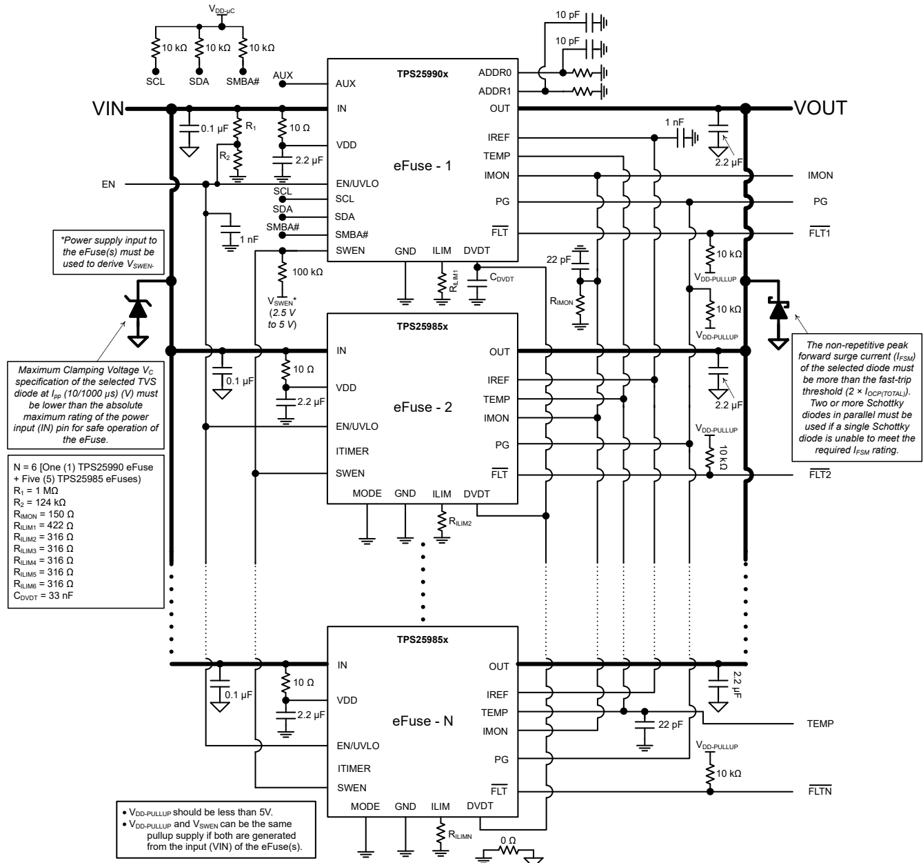
图 9-4. Application Schematic for a 12-V, 4-kW Power Path Protection Circuit with PMBus® Interface
