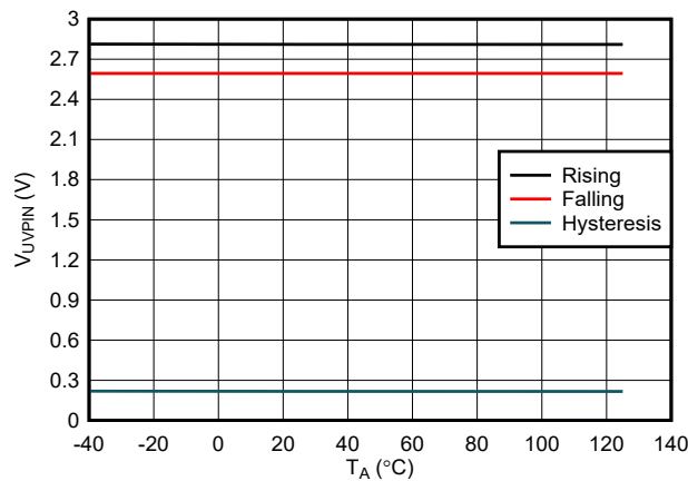
图 7-3. VIN Undervoltage Thresholds Across Temperature
