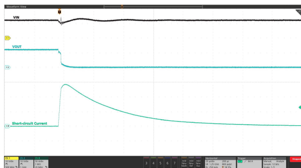
图 9-13. Output Hot-Short Response: V_{IN} = 12\text{ V} , R_{IMON} = 150\ \Omega , V_{IREF} = 1\text{ V} , and OUT Shorted to GND
