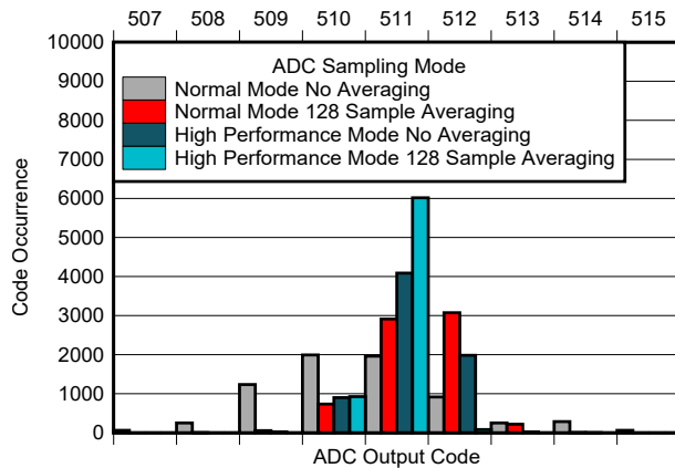
图 7-25. ADC Histogram (Mid-scale Analog Input)
