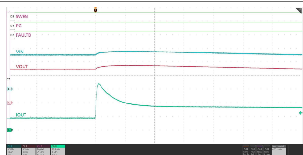
图 7-58. Short-Circuit Protection During Steady-state
