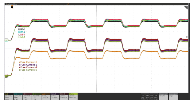
图 9-10. Transient Overload (Current distribution among six devices in parallel): V_{IN} = 12 V, t_{OC\_TIMER} = 10 ms, C_{LOAD} = 50 mF, R_{IMON} = 150 \Omega , V_{IREF} = 1 V, and Load Current Stepped from 333 A to 500 A then 333 A within 8.5 ms
