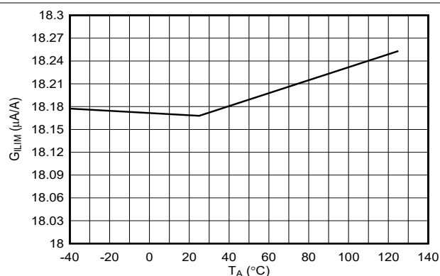
图 7-15. ILIM Gain Across Load and Temperature
