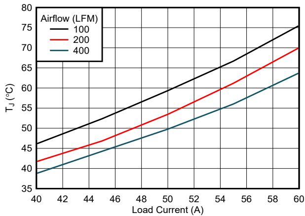
图 7-33. Junction Temperature vs Load Current (With Air-Flow)
