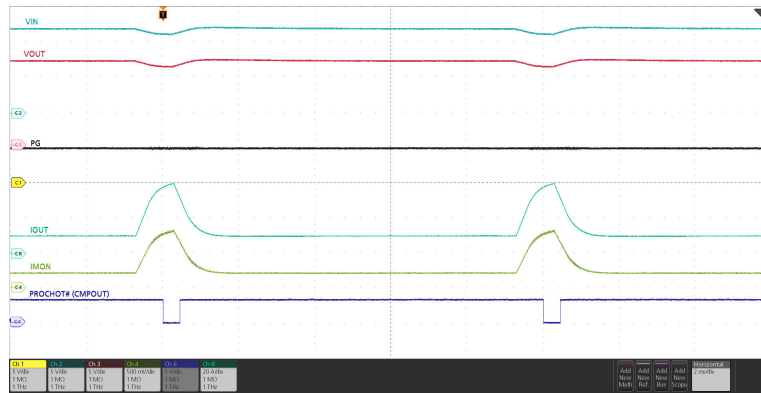
图 8-9. PROCHOT# Response Using Internal Comparator
