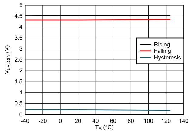
图 7-4. VIN Undervoltage Thresholds Across Temperature (VIN_UV_FLT = 0x38)
