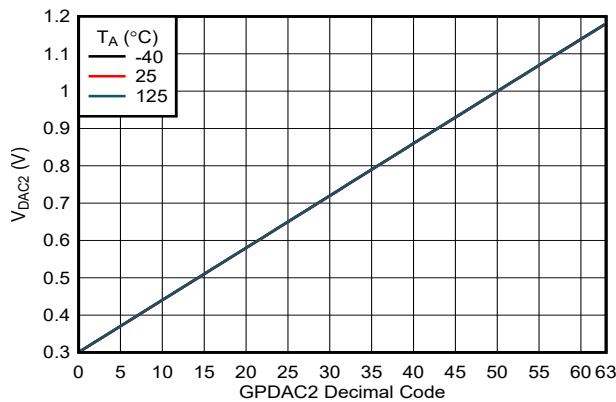
图 7-27. General Purpose DAC2 Transfer Function
