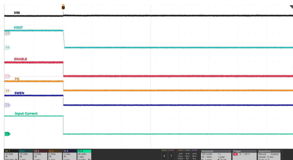
图 7-39. Power Cycle Using PMBus Command
