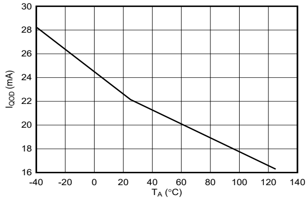
图 7-31. QOD Sink Current Across Temperature
