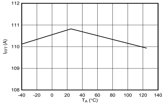
图 7-19. Fixed Fast-trip Threshold Across Temperature
