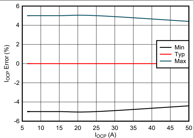
图 7-14. Steady-state Overcurrent Protection Threshold (Circuit-Breaker) Accuracy
