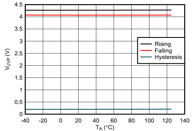
图 7-2. VDD Undervoltage Thresholds Across Temperature
