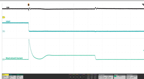
图 7-57. Short-Circuit Protection During Steady-state
