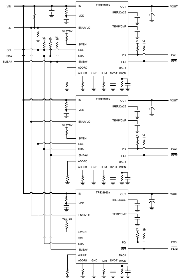
图 9-3. Multiple TPS25990 Devices Delivering Power to Different Zones in a System
