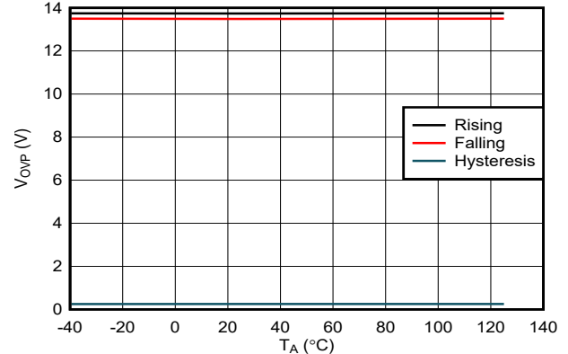
图 7-8. VIN Overvoltage Protection Threshold Across Temperature (VIN_OV_FLT = 0x0B)
