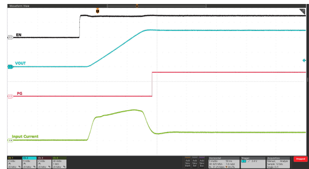
图 9-6. Start-up with EN/UVLO: V_{IN} = 12 V, EN/UVLO Stepped Up From 0 V to 3 V, C_{LOAD} = 50 mF, R_{LOAD(Start-up)} = 0.48 \Omega , C_{DVRT} = 33 nF, V_{IREF} = 1 V, R_{ILIM(TPS25990)} = 422 \Omega , and R_{ILIM(TPS25985)} = 316 \Omega
