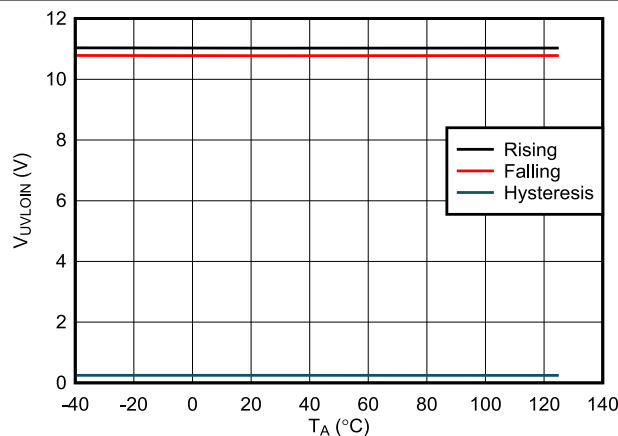
图 7-5. VIN Undervoltage Thresholds Across Temperature (VIN_UV_FLT = 0x8D)
