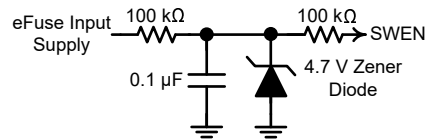
图 9-16. Zener Regulator Used as Pullup Supply for SWEN
