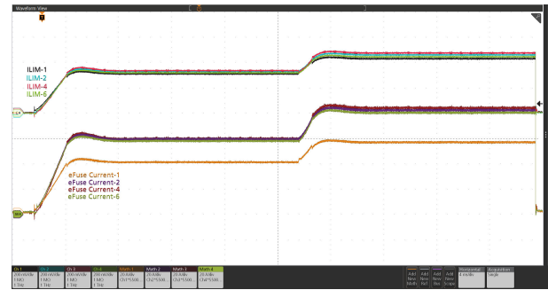
图 9-12. Circuit-Breaker Response (Current distribution among six devices in parallel): V_{IN} = 12\text{ V} , t_{OC\_TIMER} = 17\text{ ms} , C_{LOAD} = 50\text{ mF} , R_{IMON} = 150\ \Omega , V_{IREF} = 1\text{ V} , and Load Current Stepped from 333 A to 530 A for more than 17 ms
