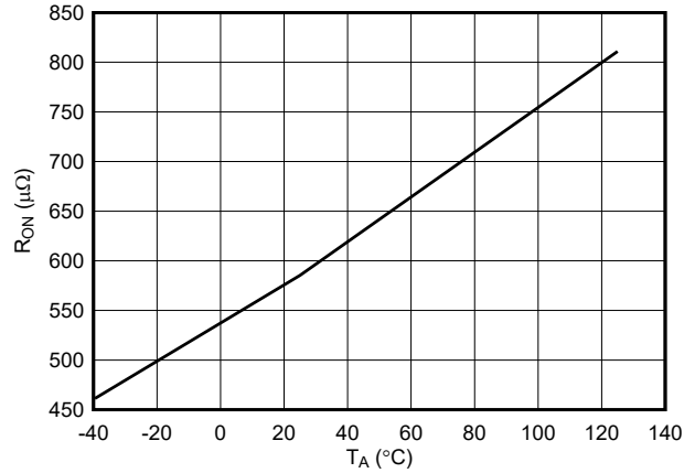
图 7-1. ON Resistance Across Temperature
