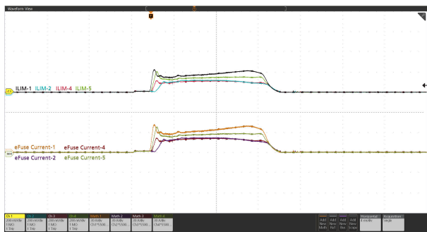
图 9-6. Start-up with EN/UVLO (Current distribution among five devices in parallel): V_{IN} = 12 V, EN/UVLO Stepped Up From 0 V to 3 V, C_{LOAD} = 55 mF, C_{DVRT} = 33 nF, R_{IREF} = 40.2 k \Omega , and R_{ILIM} on Each Device = 300 \Omega
