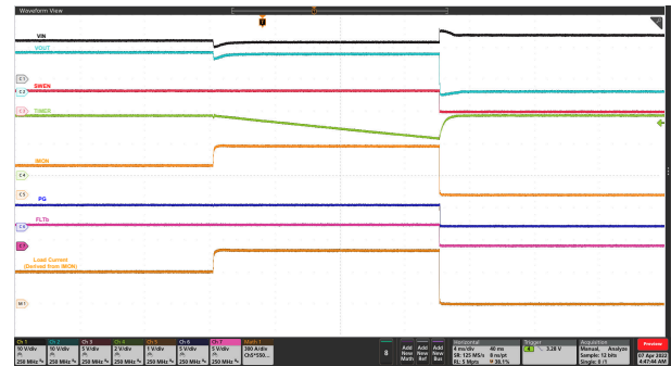
图 9-11. Circuit-Breaker Response: V_{IN} = 12\text{ V} , C_{ITIMER} = 22\text{ nF} , C_{LOAD} = 55\text{ mF} , R_{IMON} = 167\text{ }\Omega , R_{REF} = 40.2\text{ k}\Omega , and Load Current Stepped up From 300 A to 500 A for > 20 ms
