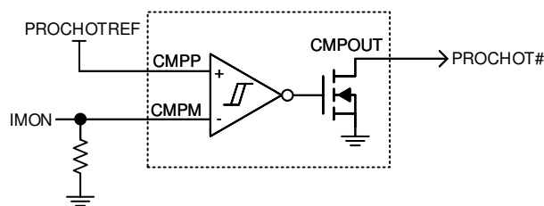
图 8-9. Adjustable Fast Overcurrent (PROCHOT#) Detect Using Internal Comparator
