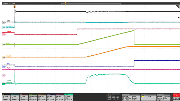
图 9-4. Input Hot Plug: V_{IN} Stepped Up from 0 V to 12 V, C_{LOAD} = 55 mF, C_{DVRT} = 33 nF, R_{IREF} = 40.2 k \Omega , and R_{ILIM} on Each Device = 300 \Omega
