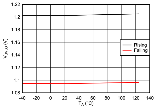
图 7-5. EN/UVLO Thresholds Across Temperature
