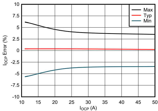
图 7-11. Steady-State Overcurrent Protection Threshold (Circuit-Breaker) Accuracy
