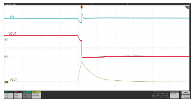
图 9-13. Output Hot-Short Response: V_{IN} = 12\text{ V} , R_{IMON} = 167\text{ }\Omega , R_{REF} = 40.2\text{ k}\Omega , and OUT Shorted to GND
