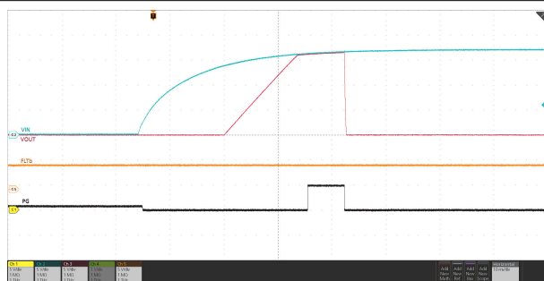
图 7-29. Input Overvoltage Protection Response
