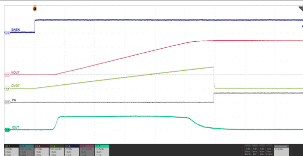
图 7-27. Inrush Current Control with Capacitive Load
