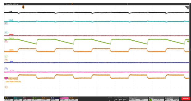
图 9-9. Transient Overload: V_{IN} = 12 V, C_{TIMER} = 22 nF, C_{LOAD} = 55 mF, R_{IMON} = 167 \Omega , R_{IREF} = 40.2 k \Omega , and Load Current Stepped from 300 A to 400 A then 300 A within 10 ms
