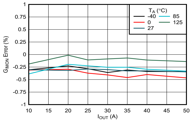
图 7-9. IMON Gain Accuracy Across Load and Temperature
