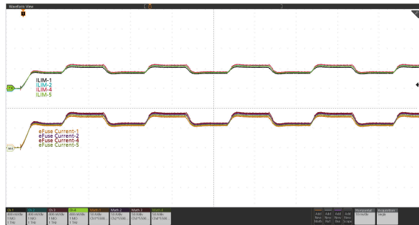
图 9-10. Transient Overload (Current distribution among five devices in parallel): V_{IN} = 12\text{ V} , C_{ITIMER} = 22\text{ nF} , C_{LOAD} = 55\text{ mF} , R_{IMON} = 167\text{ }\Omega , R_{REF} = 40.2\text{ k}\Omega , and Load Current Stepped from 300 A to 450 A then 300 A within 8.5 ms
