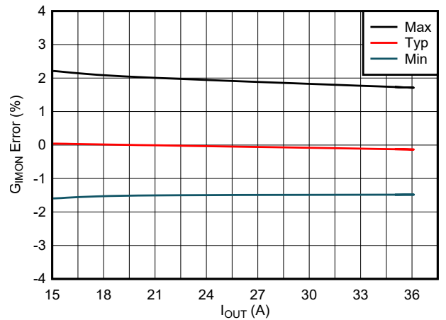
图 7-10. IMON Gain Accuracy Across Process and Temperature Corners
