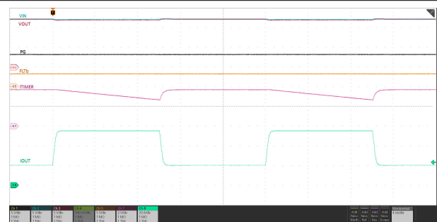
图 7-28. Inrush Current Control with Capacitive and Resistive Load
