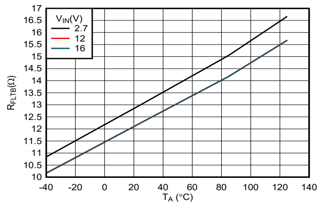
图 7-23. \overline{\text{FLT}} Pin Pulldown Resistance vs Temperature
