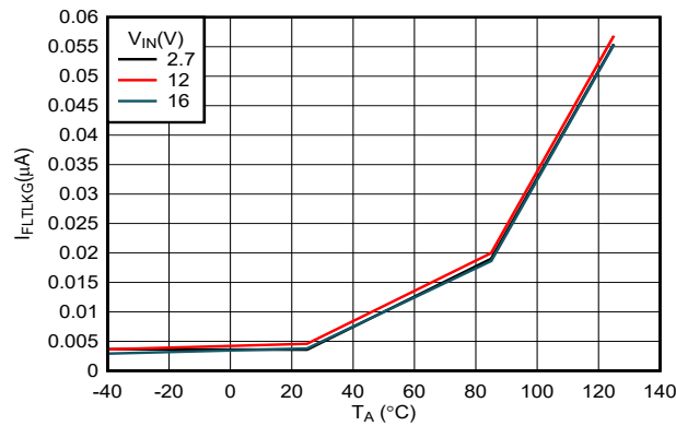
图 7-24. \overline{\text{FLT}} Pin Leakage Current vs Temperature
