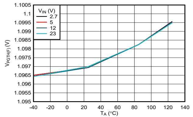
图 6-26. PGTH Threshold (Falling) vs Temperature (TPS25972x, TPS25974x Variants)
