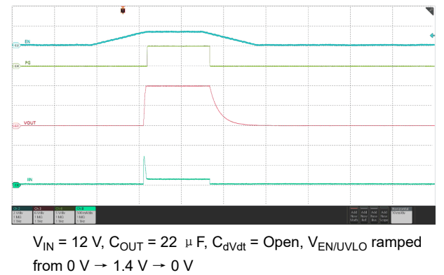
图 6-30. Power Up and Down With EN/UVLO Control
