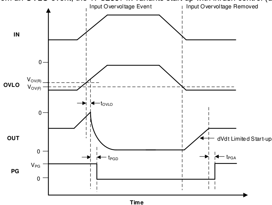
图 7-7. TPS25974x Overvoltage Lockout and Recovery
