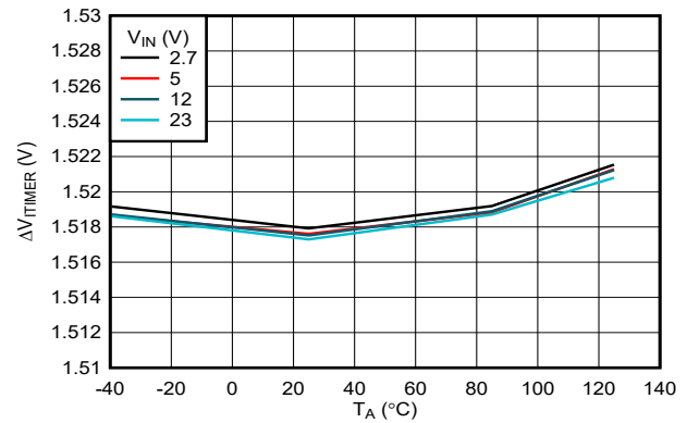
图 6-20. ITIMER Discharge Differential Voltage Threshold vs Temperature
