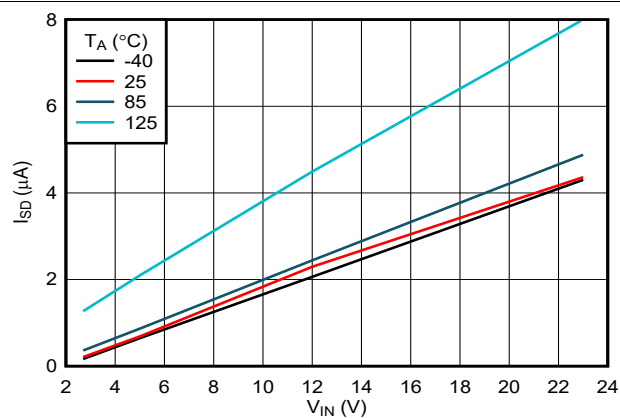
图 6-5. IN Shutdown Current vs Temperature
