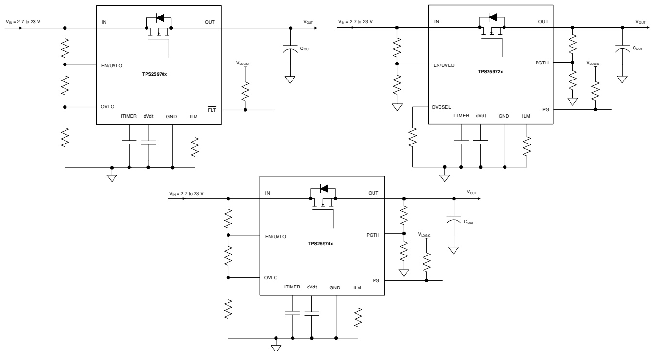
图 8-1. Single Device, Self-Controlled
