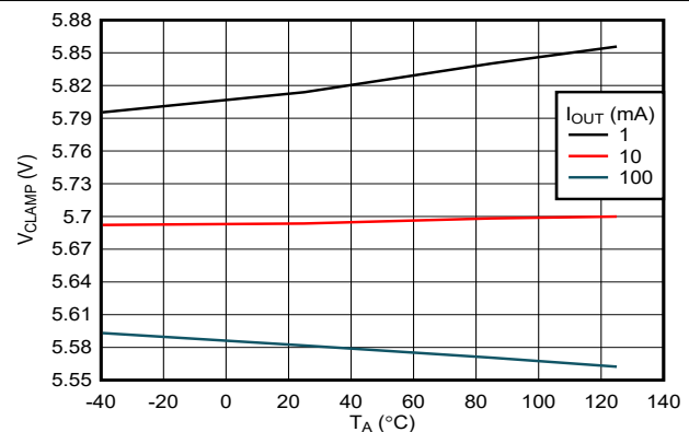
图 6-18. OVC Clamping Voltage (OVCSEL = OPEN) vs Load Current (TPS25972x Variant)
