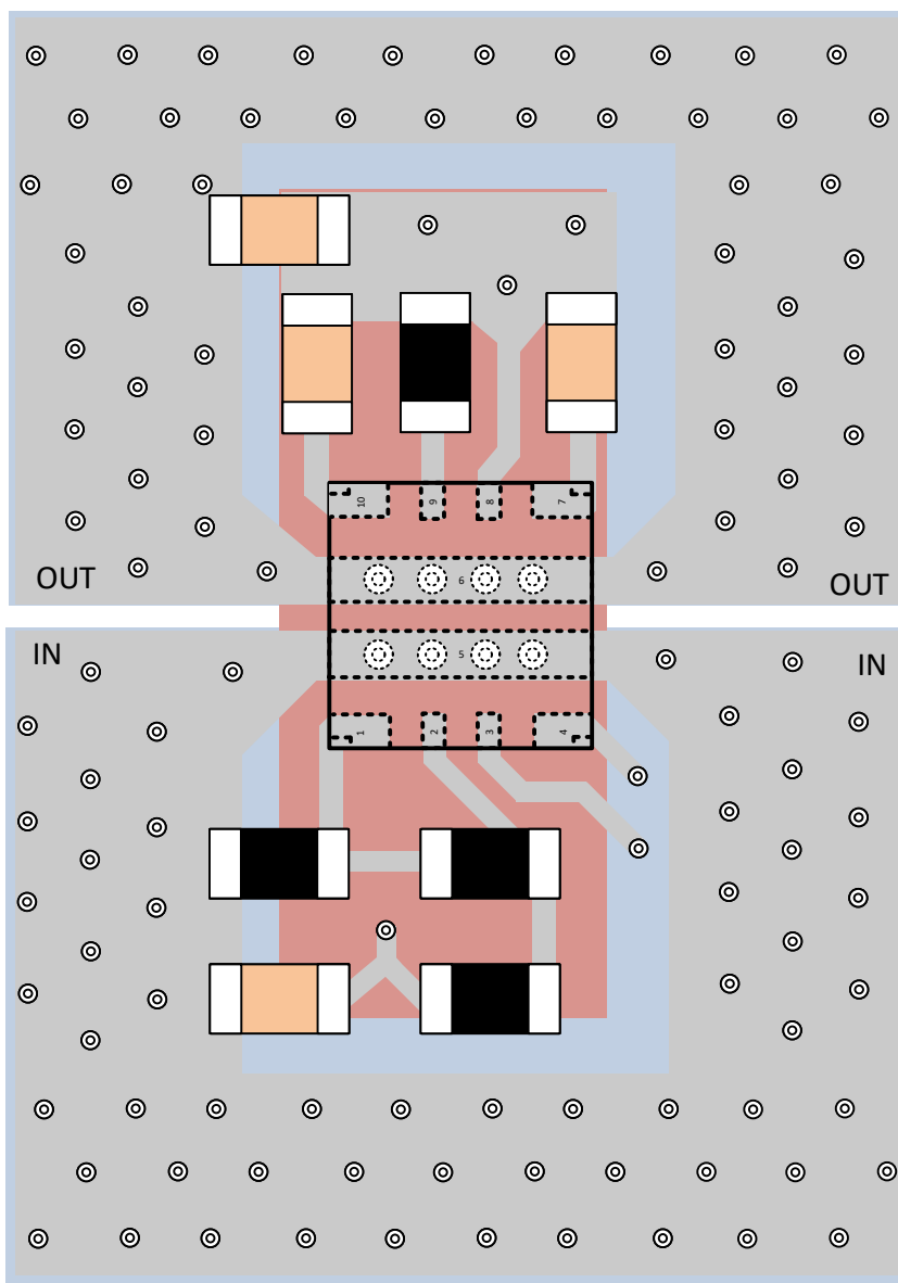
图 8-11. Layout Example - Single TPS25974x With PGTH Referred to OUT
