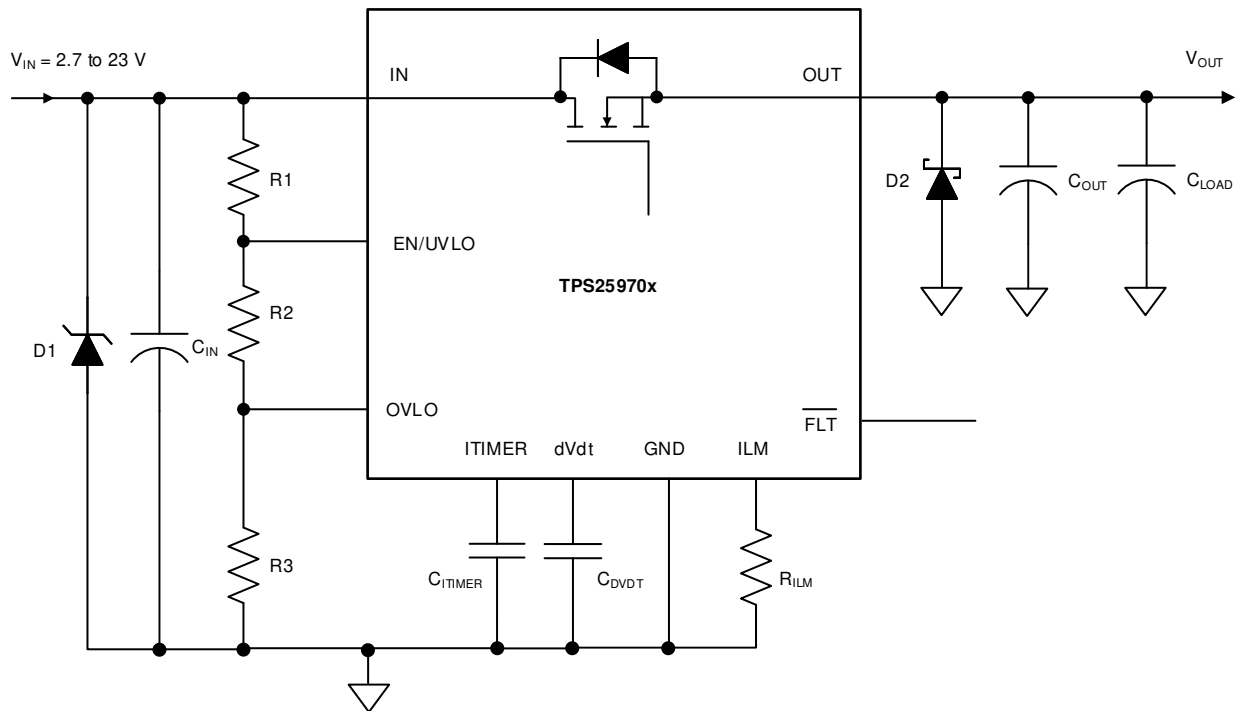
图 8-10. Circuit Implementation With Optional Protection Components
