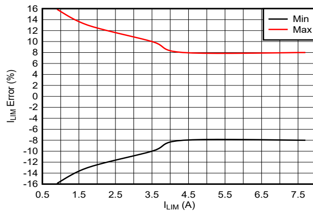
图 6-13. Overcurrent Threshold Accuracy (Across Process, Voltage and Temperature)
