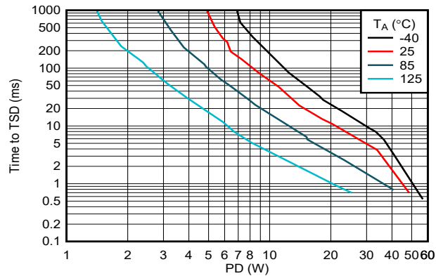
图 6-29. Time to Thermal Shut-Down During Steady State
