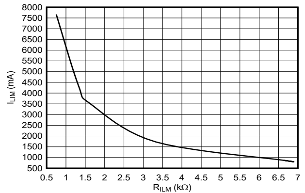
图 6-12. Overcurrent Threshold vs ILM Resistor
