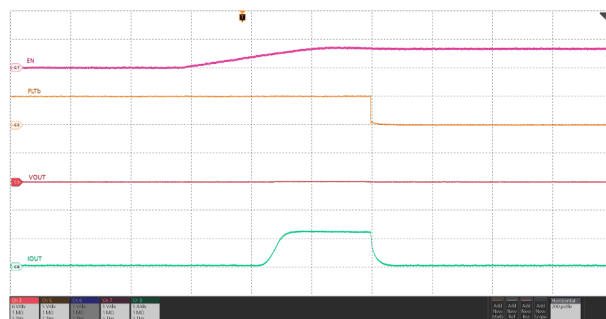
图 6-44. Output Short-Circuit During Steady State
