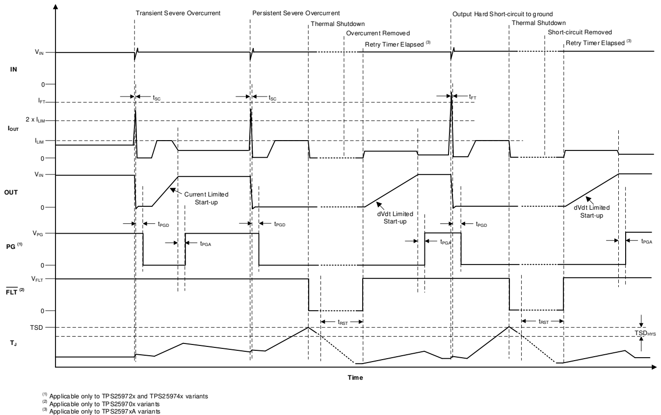
图 7-11. TPS2597xx Short-Circuit Response
