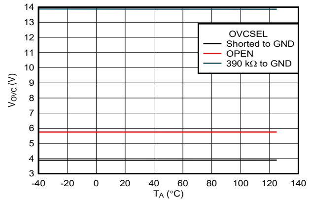
图 6-16. OVC Threshold vs Temperature (TPS25972x Variant)
