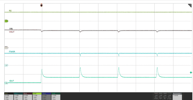
图 8-5. Transient Overload
