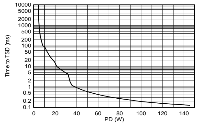
图 6-28. Time to Thermal Shut-Down During Inrush State
