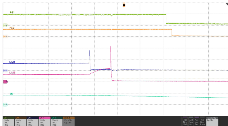
图 8-9. Parallel Devices Load Current During Steady State and Overload
