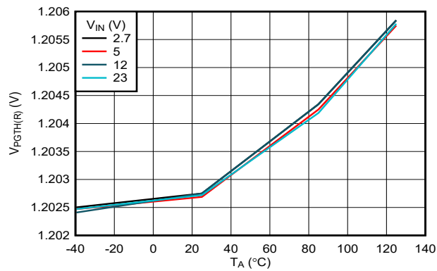
图 6-25. PGTH Threshold (Rising) vs Temperature (TPS25972x, TPS25974x Variants)
