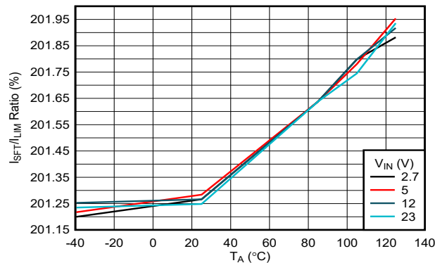
图 6-15. Scalable Fast-Trip Threshold: Current Limit Threshold ( I_{LIM} ) Ratio vs Temperature
