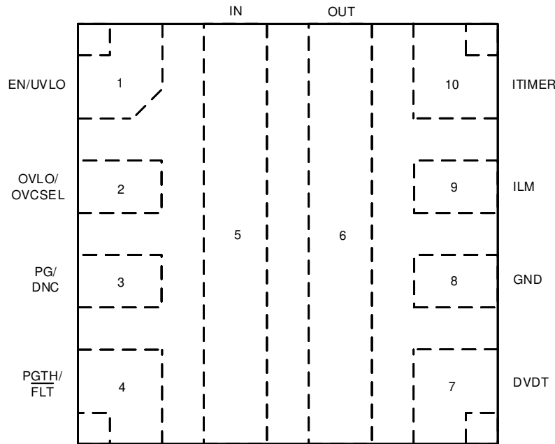
图 5-1. TPS2597xx RPW Package 10-Pin QFN (Top View)
