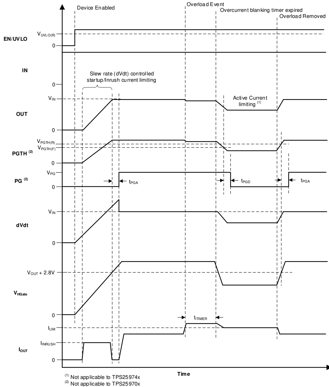
图 7-13. TPS25972x, TPS25974x PG Timing Diagram
