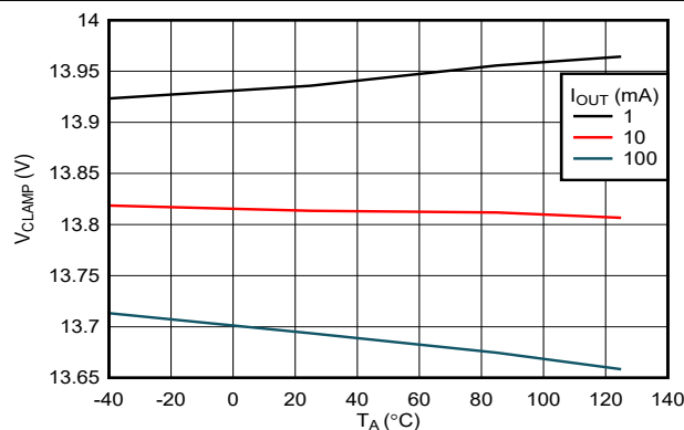
图 6-17. OVC Clamping Voltage (OVCSEL = 390 kΩ to GND) vs Load Current (TPS25972x Variant)
