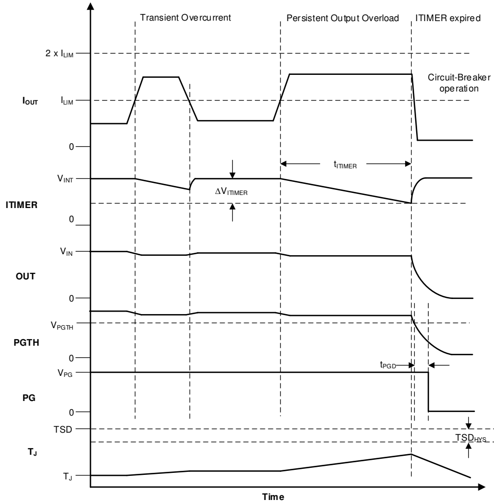
图 7-9. TPS25974x Overcurrent Response
