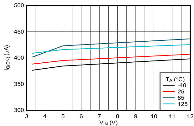
图 6-3. IN Quiescent Current vs Temperature (TPS25972x Variant)
