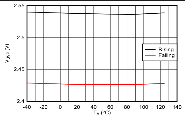
图 6-6. IN Undervoltage Threshold vs Temperature
