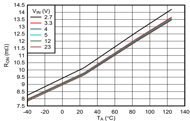
图 6-1. ON-Resistance vs Supply Voltage
