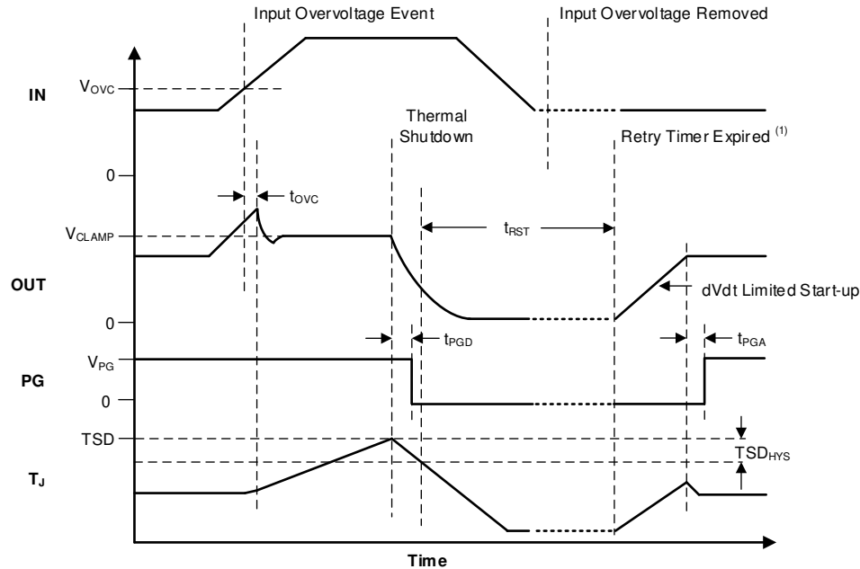
图 7-8. TPS25972x Overvoltage Response (Auto-Retry)
