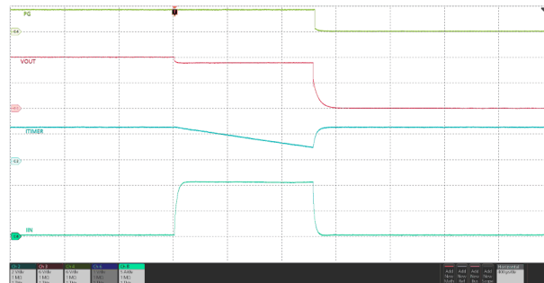
图 8-6. Circuit Breaker Response
