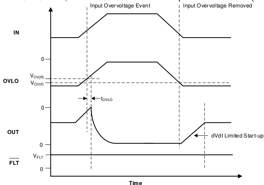
图 7-6. TPS25970x Overvoltage Lockout and Recovery
