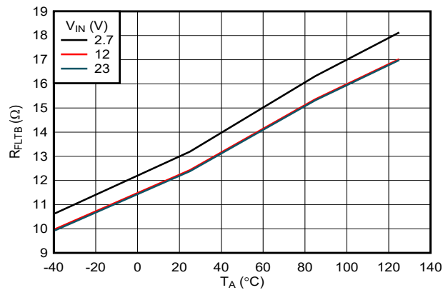
图 6-27. FLT Pin Pulldown Resistance vs Temperature
