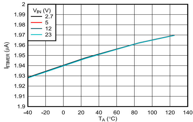
图 6-21. ITIMER Discharge Current vs Temperature
