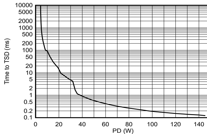
图 8-3. Thermal Shut-Down Plot During Inrush
