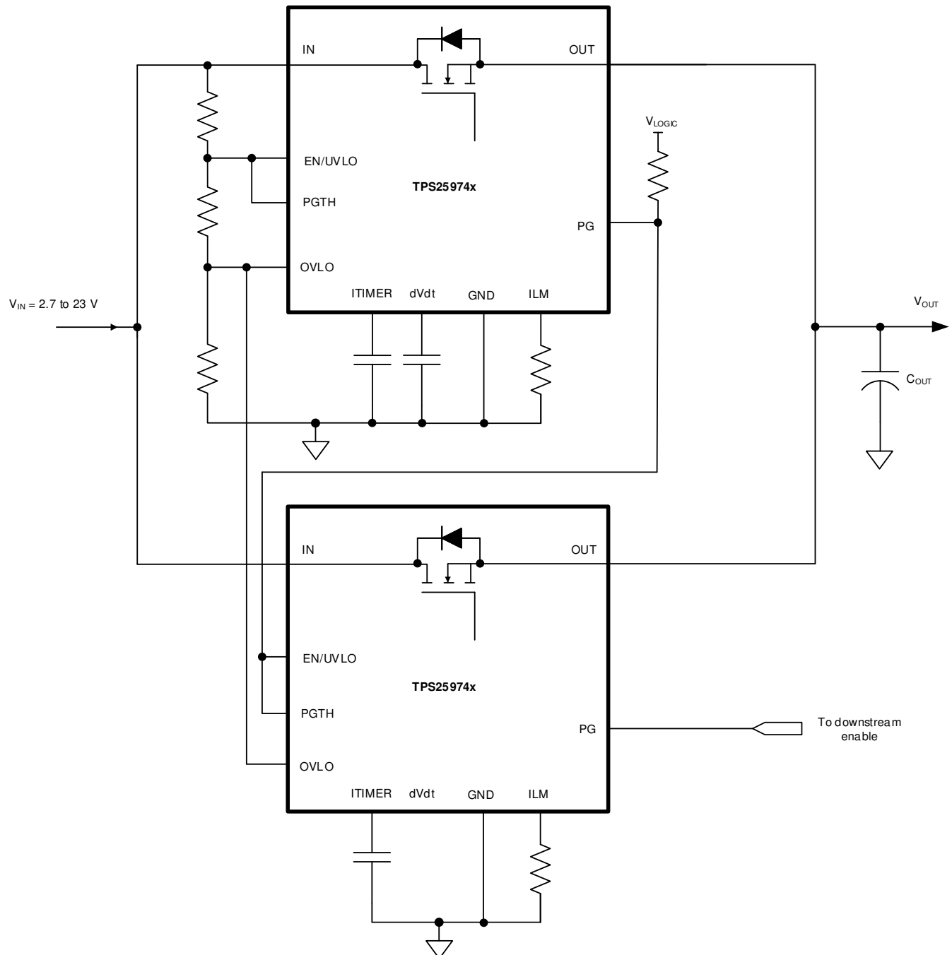
图 8-7. Two Devices Connected in Parallel for Higher Steady State Current Capability
