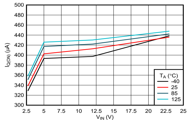
图 6-2. IN Quiescent Current vs Temperature (TPS25970x, TPS25974x Variants)
