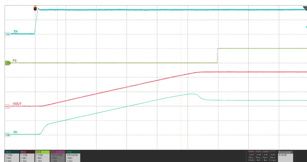
图 6-33. Inrush Current Without Slew Rate Control - Capacitive Load
