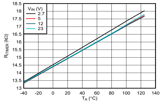
图 6-22. ITIMER Internal Pullup Resistance vs Temperature
