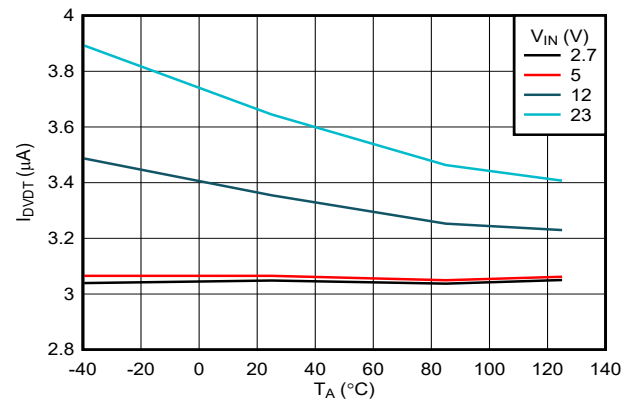
图 6-24. DVDT Charging Current vs Temperature
