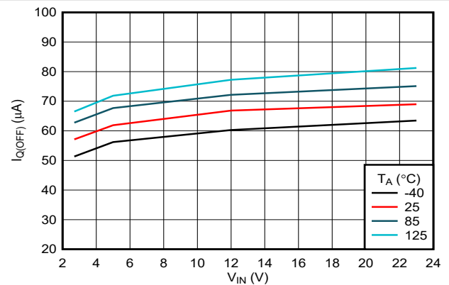
图 6-4. IN OFF State (UVLO) Current vs Temperature
