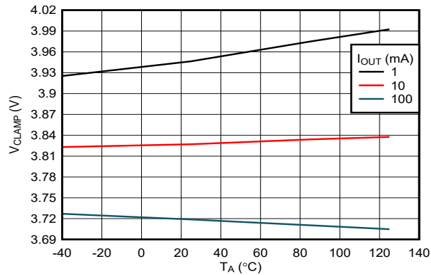
图 6-19. OVC Clamping Voltage (OVCSEL = GND) vs Load Current (TPS2597x Variant)
