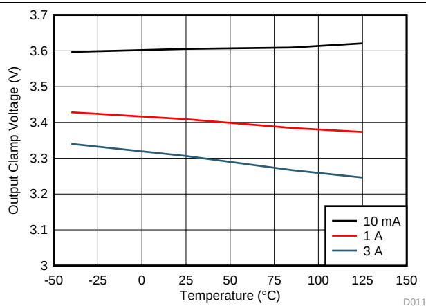
图 10. OVC Threshold vs Temperature
