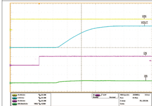
图 28. Output Voltage Ramp and Inrush Current at Start Up, C_{dvdt} = \text{Open}
