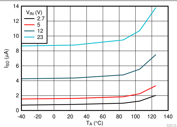
图 7-7. IN Shutdown Current vs Temperature
