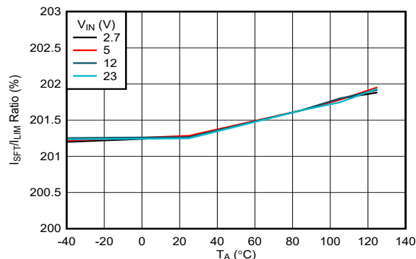
图 7-17. Scalable Fast-Trip Threshold: Current Limit Threshold ( I_{LIM} ) Ratio vs Temperature
