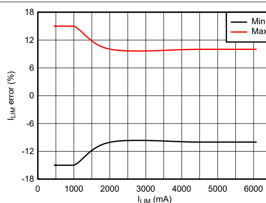
图 7-15. Overcurrent Threshold Accuracy (Across Process, Voltage and Temperature)
