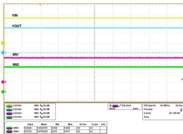
图 9-20. Parallel Devices Load Current During Steady State
