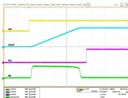
图 7-39. Start-Up with Supply
