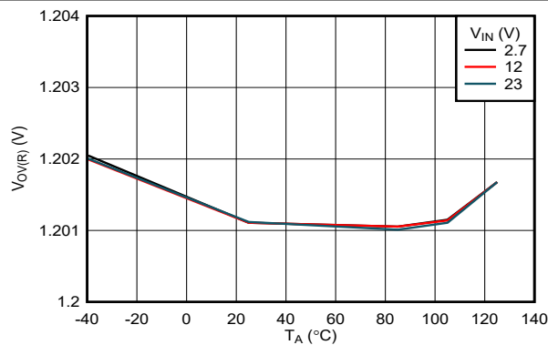
图 7-12. OVLO Rising Threshold vs Temperature
