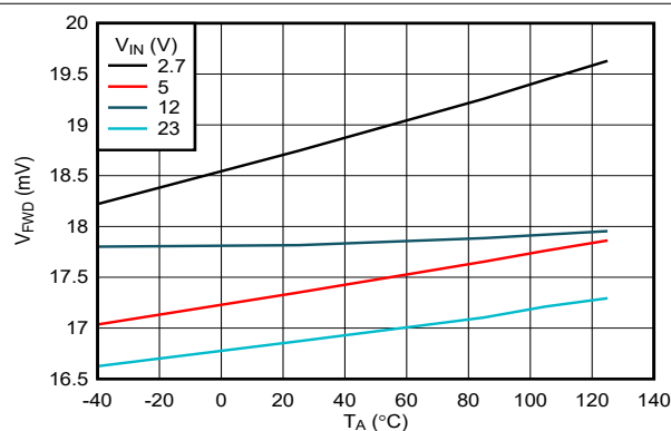
图 7-19. RCB - Forward Regulation Voltage vs Temperature
