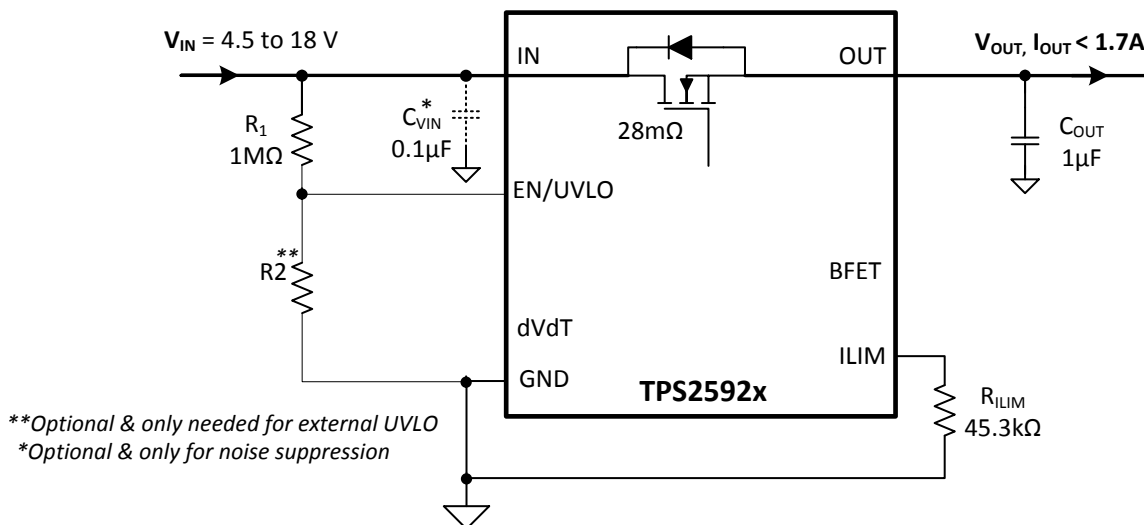
Figure 28. Typical Application Schematic: Simple e-Fuse for STBs
