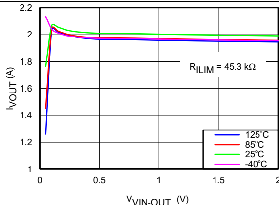
Figure 14. I_{\text{OUT}} vs V_{\text{VIN-OUT}}
