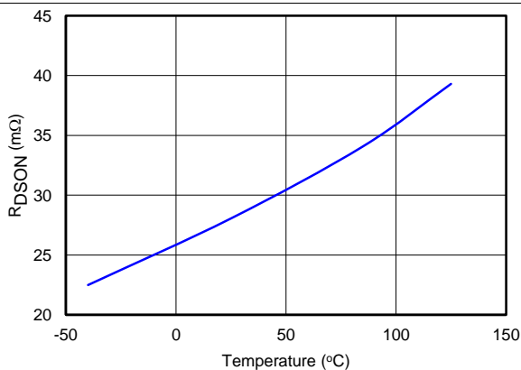
Figure 13. R_{\text{DS(on)}} vs Temperature
