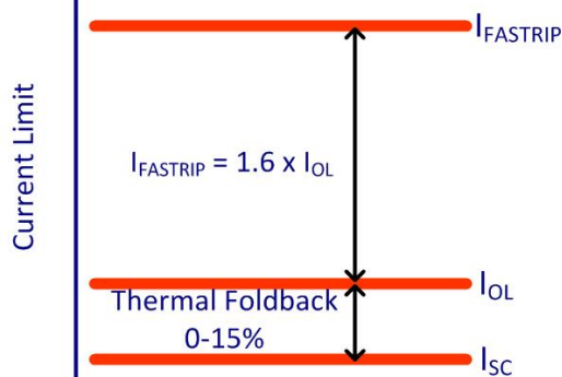
Figure 26. Fast-Trip Current
