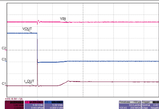
Figure 27. Fast-Trip and Current Limit Amplifier Response for Short Circuit
