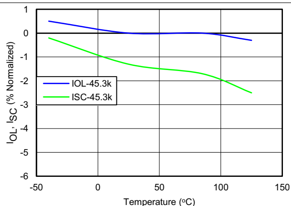
Figure 14. I_{OL} , I_{SC} vs Temperature
