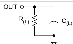
图 9-1. OUT Rise-Fall Test Load Figure
