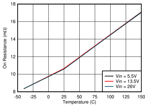
图 8-11. Low-side MOSFET on Resistance vs Junction Temperature
