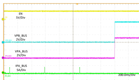
图 11-23. Short Circuit Recovery
