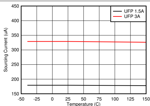
图 8-23. CC Sourcing Current vs Junction Temperature
