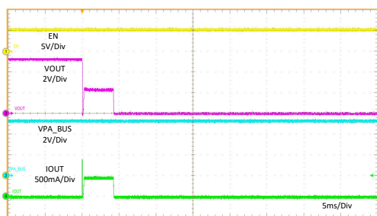
图 11-28. OUT short to 5.1- \Omega Load
