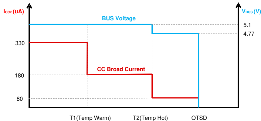
图 10-17. TPS25850-Q1 Behavior When Trigger Temp Warm/Hot Threshold
