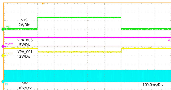
图 11-30. Thermal Sensing - NTC Temperature WARM Behavior
