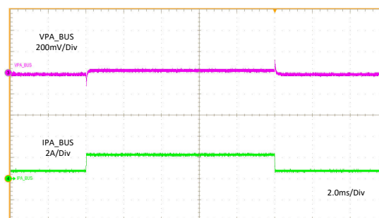
图 11-9. Load Transient Without Cable Compensation
