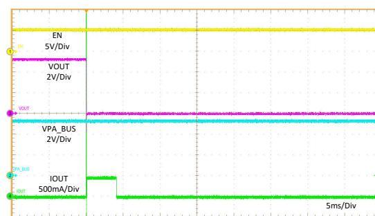
图 11-27. PA_CC2 Hot Short to GND
