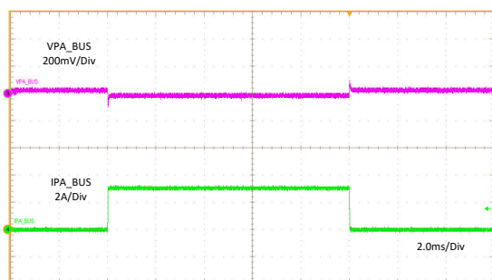
图 11-8. Load Transient Without Cable Compensation
