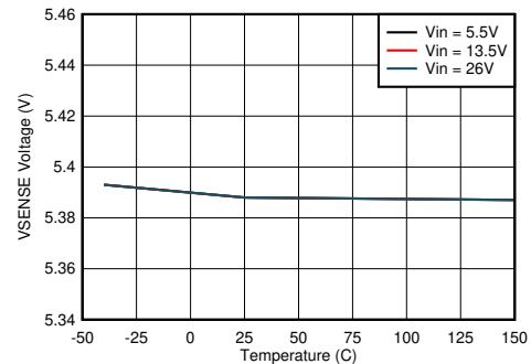
图 8-6. V_{SENSE} Voltage vs Junction Temperature
