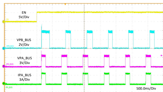
图 11-22. Enable Into Short
