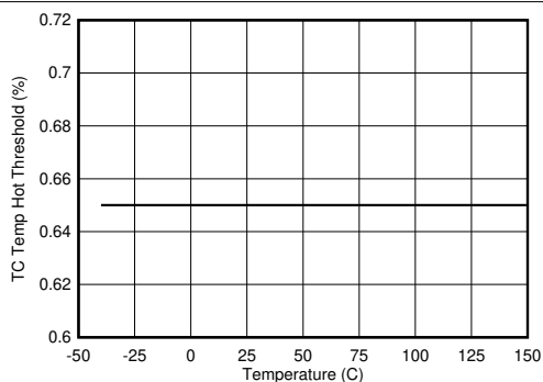
图 8-25. TS Temperature Hot Threshold vs Junction Temperature
