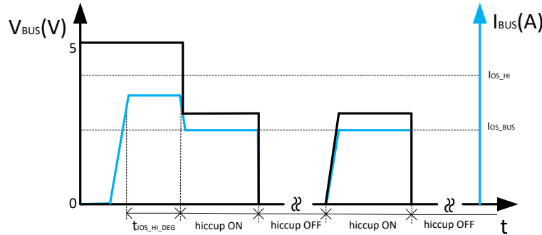
图 10-12. BUS Overcurrent Protection
