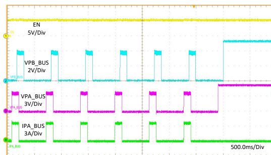
图 11-25. 1- \Omega Load Recovery
