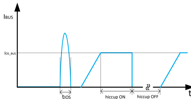
图 10-11. Response Time to BUS Short-Circuit
