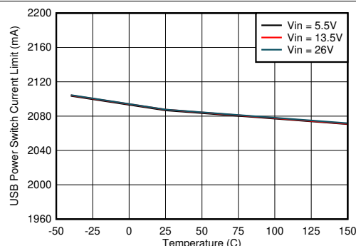
图 8-14. USB Power Switch Current Limit vs Junction Temperature
