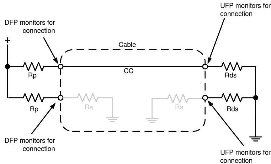
图 10-20. DFP-UFP Connection
