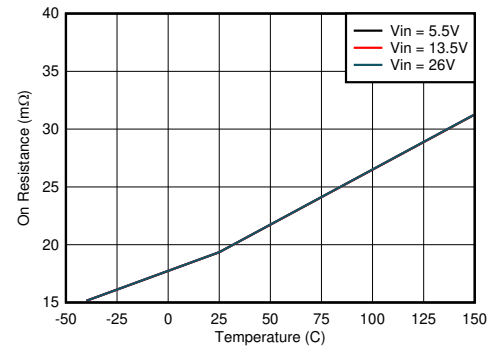
图 8-10. High-side MOSFET on Resistance vs Junction Temperature
