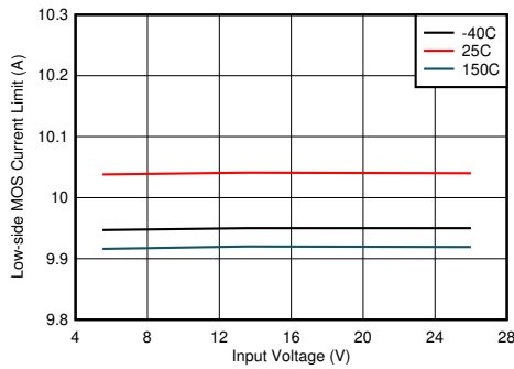
图 8-9. Low-side Current Limit vs Input Voltage
