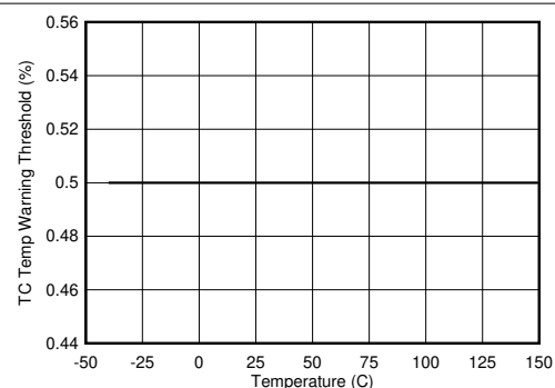
图 8-24. TS Temperature Wam Threshold vs Junction Temperature
