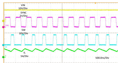
图 10-10. Synchronizing to External 2.2-MHz Clock
