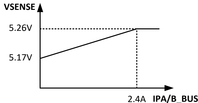
图 10-15. Dual Ports Cable Compensation
