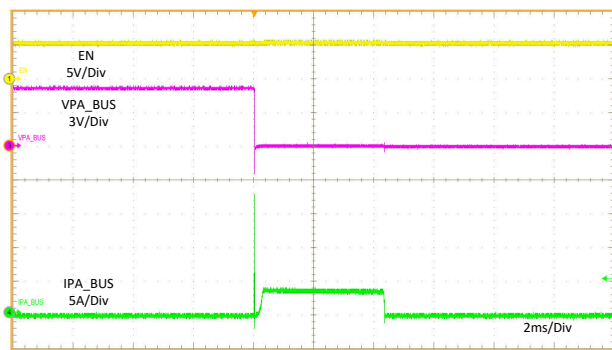
图 11-26. VBUS Hot Short to GND
