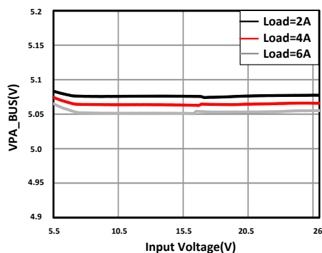
图 11-12. Dropout Characteristic
