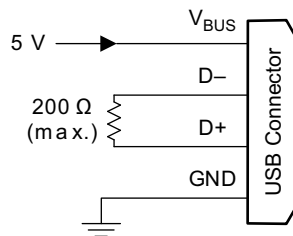
图 10-21. DCP Supporting BC1.2 and YD/T 1591-2009
