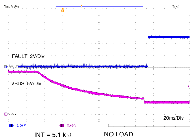
图 11-29. VBUS Short to BAT Recovery With External FET
