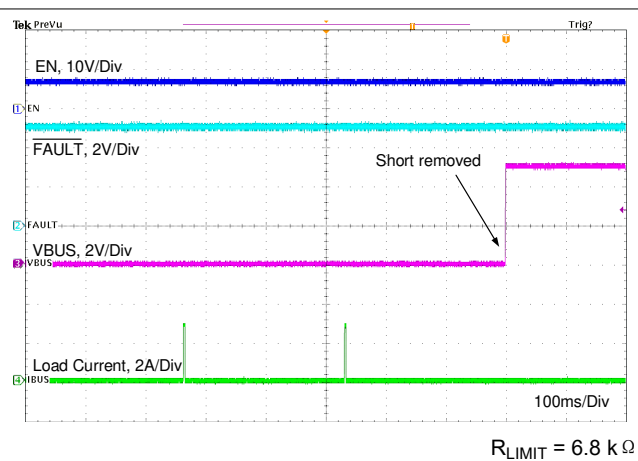
图 11-25. Short Circuit Recovery With External FET
