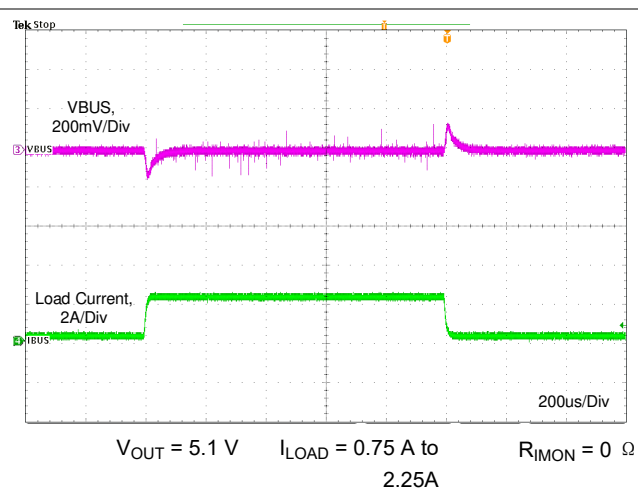
图 11-9. Load Transient Without Cable Compensation
