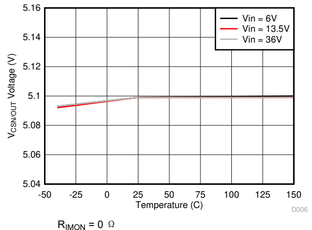
图 8-6. V_{CSN/OUT} Voltage vs Junction Temperature
