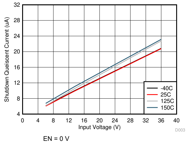
图 8-2. Shutdown Quiescent Current
