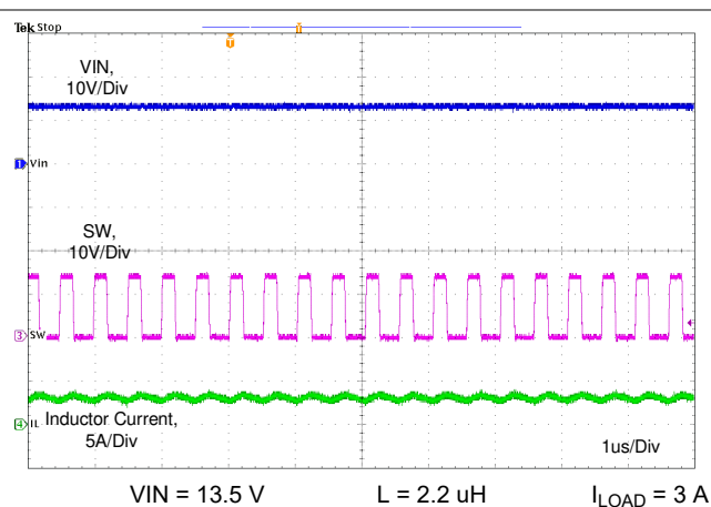
图 10-9. Switching Frequency When R_T = 8.87 \text{ k}\Omega
