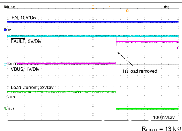
图 11-23. 1-Ω Load Recovery Without External FET
