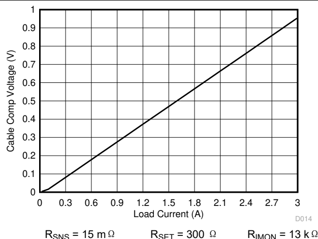
图 8-17. Cable Compensation Voltage vs Load Current
