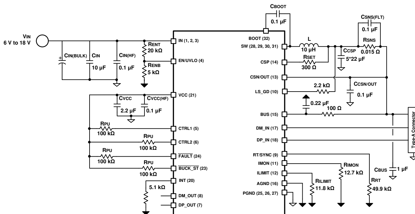
图 11-1. Application Circuit
