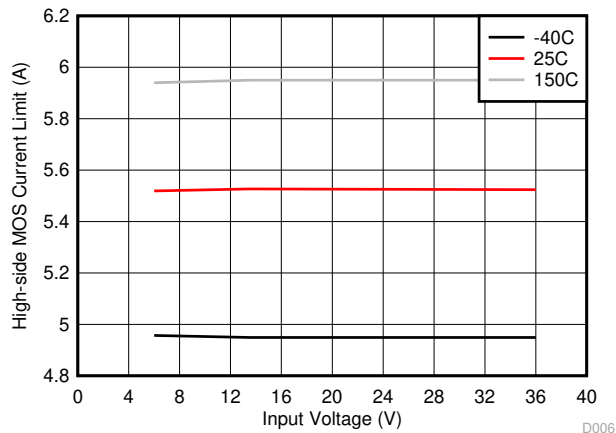
图 8-7. High-side Current Limit vs Input Voltage
