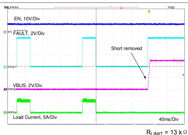
图 11-21. Short Circuit Recovery Without External FET
