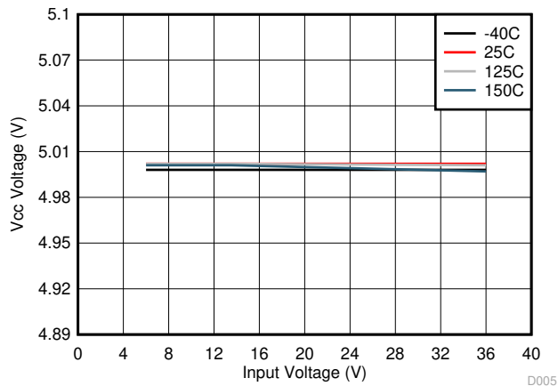
图 8-5. VCC vs Input Voltage
