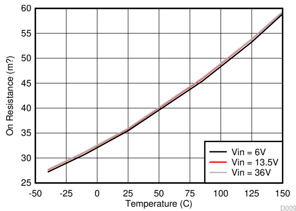
图 8-9. Low-side MOSFET on Resistance vs Junction Temperature
