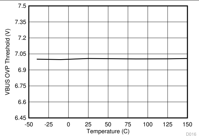
图 8-18. VBUS Overvoltage Protection Threshold vs Junction Temperature
