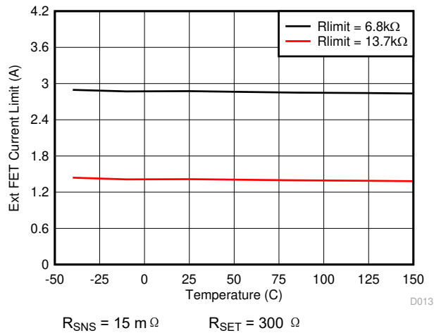
图 8-13. External FET Current Limit vs Junction Temperature
