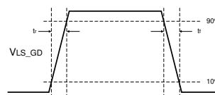
图 9-2. NFET Gate Drive Rise and Fall Time
