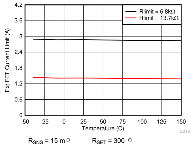
图 8-14. External FET Current Limit vs Junction Temperature
