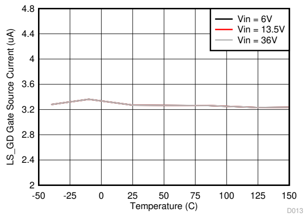
图 8-15. LS_GD Gate Source Current vs Junction Temperature
