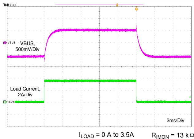
图 11-10. Load Transient With Cable Compensation
