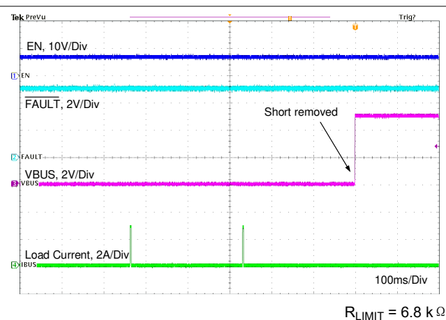
图 11-27. Short Circuit Recovery With External FET
