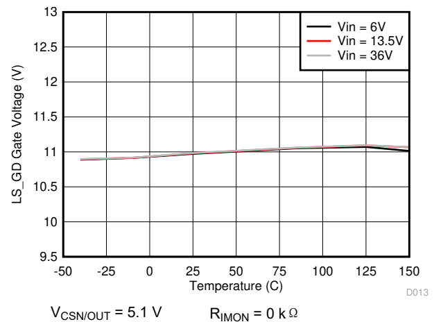
图 8-16. LS_GD Gate Voltage vs Junction Temperature
