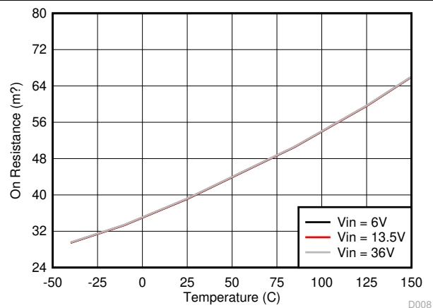
图 8-9. High-side MOSFET on Resistance vs Junction Temperature
