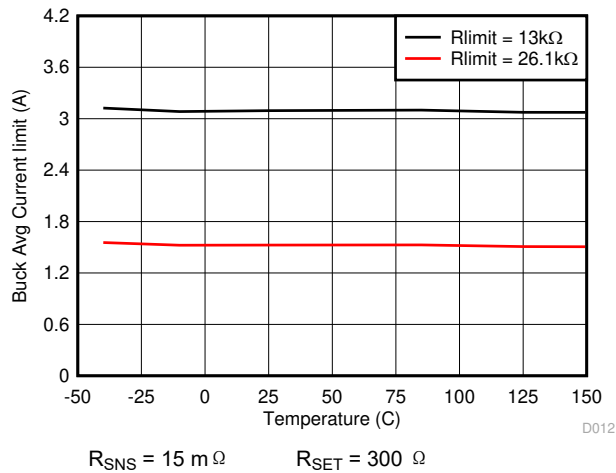
图 8-13. Buck Average Current Limit vs Junction Temperature
