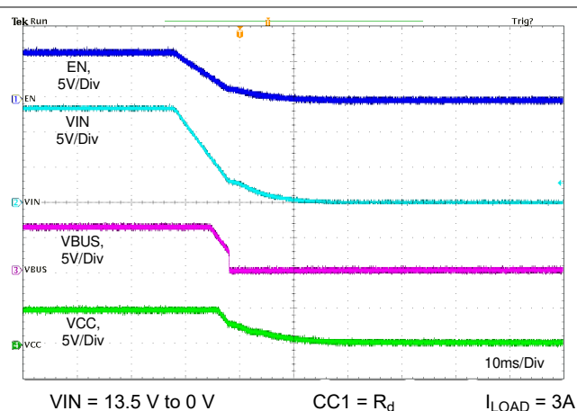
图 11-17. Shutdown Relate to VIN
