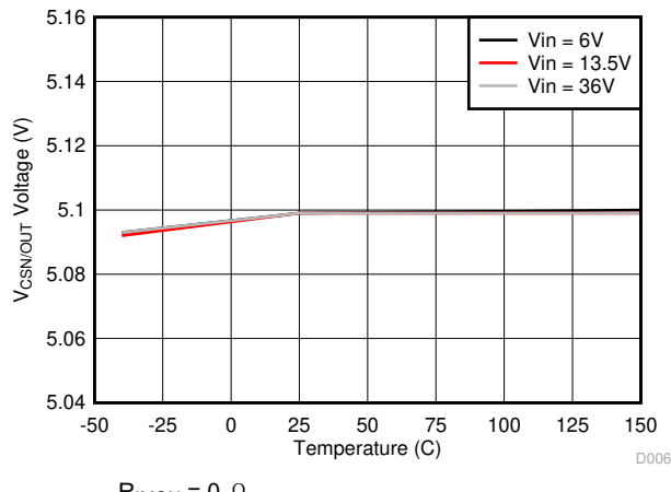
图 8-7. V_{CSN/OUT} Voltage vs Junction Temperature
