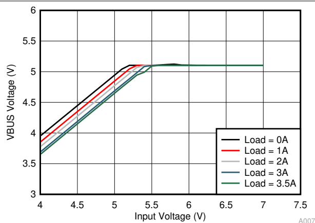
图 11-12. Dropout Characteristic
