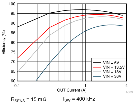
图 11-4. Efficiency With Sense Resistor
