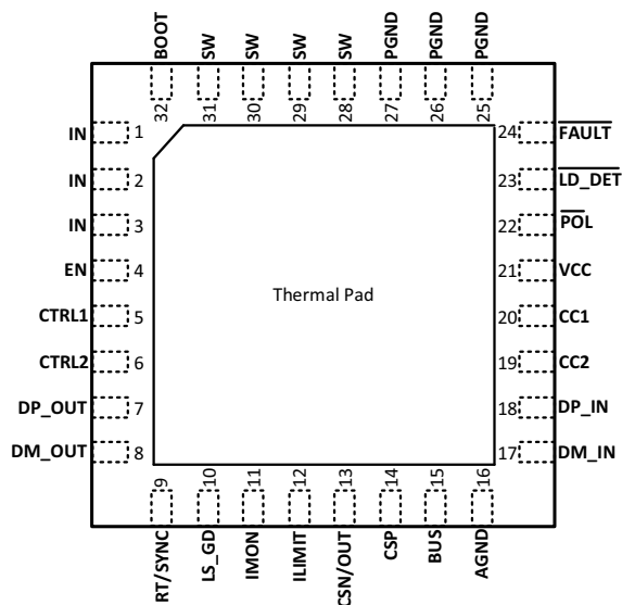
图 7-2. TPS2583xAQCWRHBRQ1 Package 32-Pin (VQFN) Top View (2)
