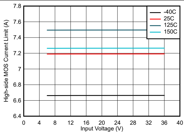
图 8-8. High-Side Current Limit vs Input Voltage
