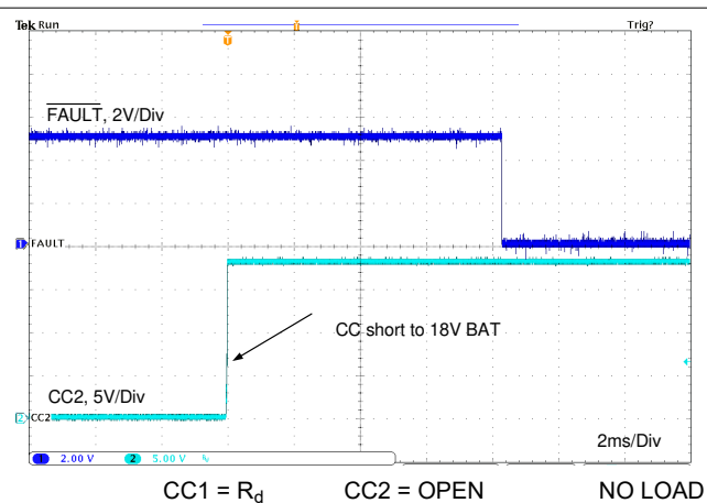
图 11-37. CC Short to BAT
