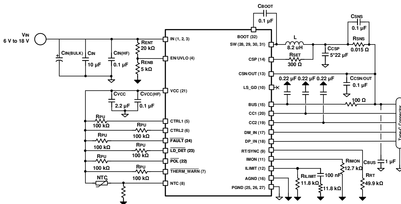
图 11-1. Application Circuit
