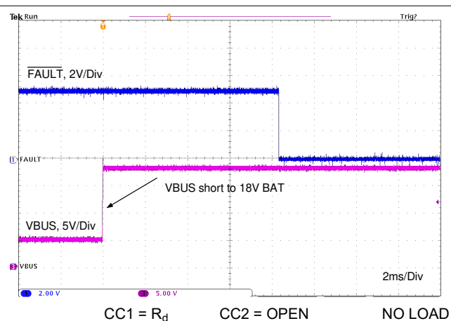
图 11-35. VBUS Short to BAT with External FET
