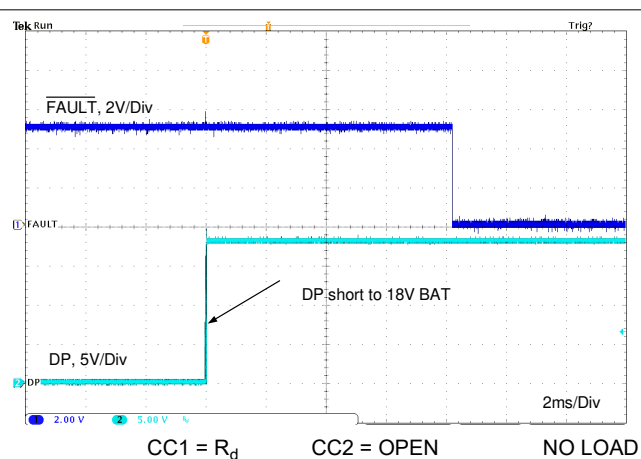
图 11-35. DP Short to BAT
