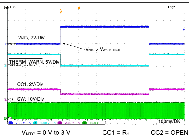
图 11-37. Thermal Sensing With NTC Behavior 1
