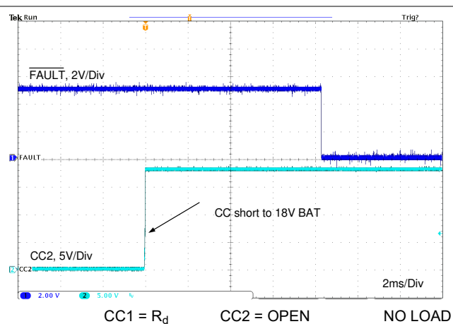
图 11-33. CC Short to BAT
