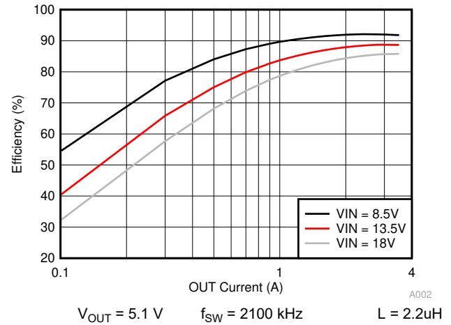
图 11-3. Buck Only Efficiency
