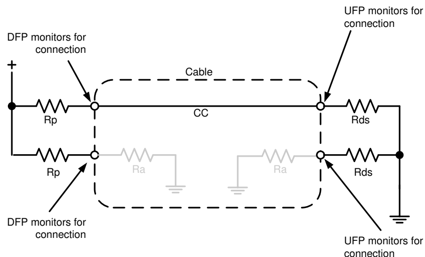
图 10-25. DFP-UFP Connection
