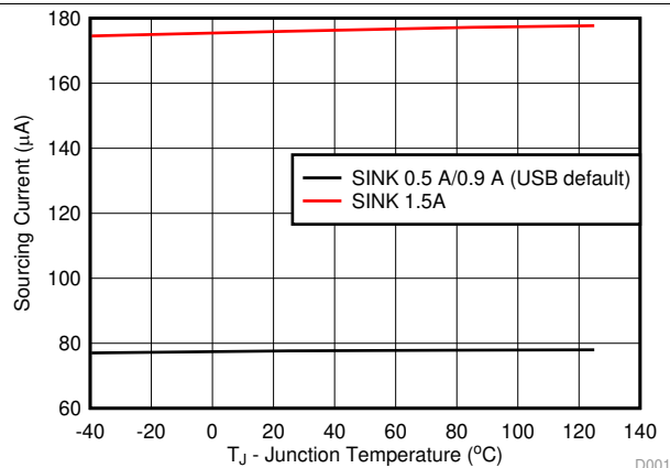
图 2. CC Sourcing Current to SINK vs Temperature
