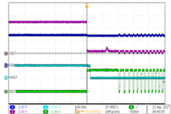
图 16. Extended Period OUT Short Event
