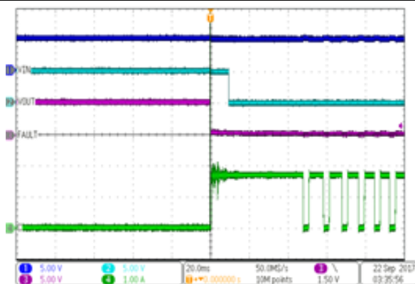
图 15. Out Short Event
