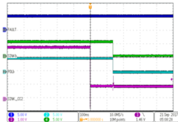
图 13. Sink Attach Event
