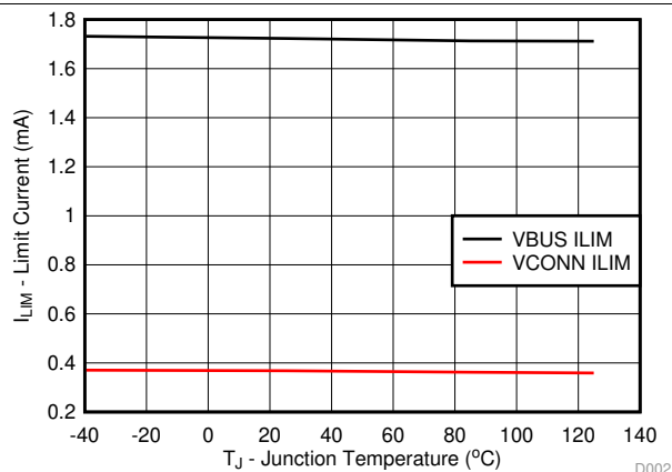
图 3. ILIM for VBUS and VCONN vs Temperature
