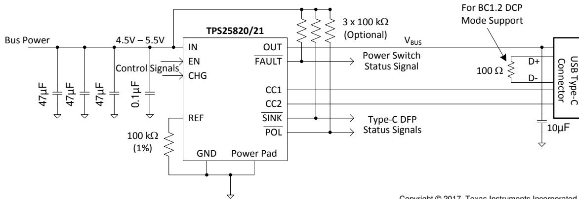
图 19. Type-C Source Port Implementation with BC 1.2 (DCP Mode) Support
