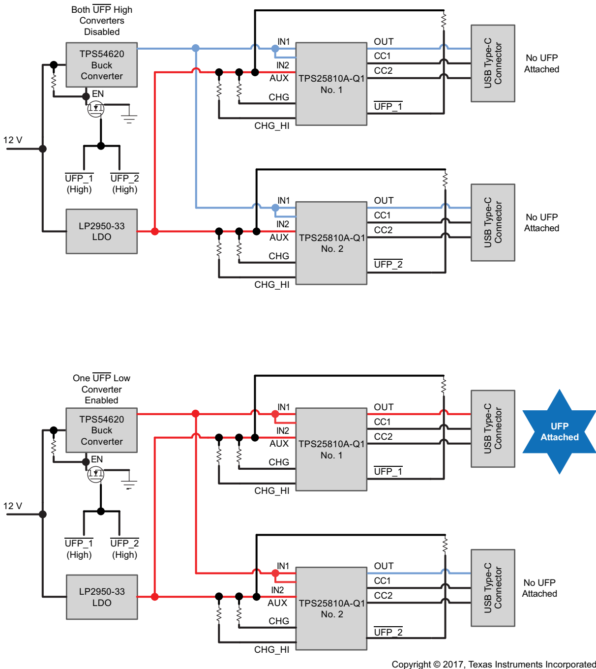
Figure 18. Power-Wake Implementation
