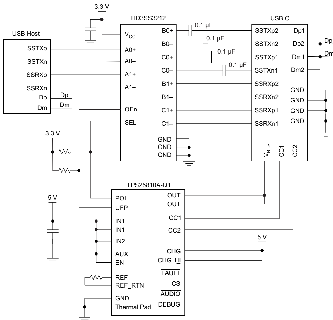
Figure 15. Example Implementation
