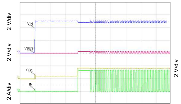
Figure 21. Start-Up
