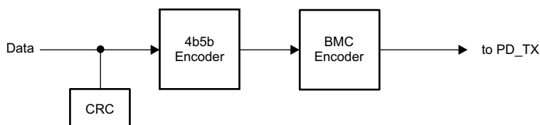
图 9-19. USB-PD Baseband Transmitter Block Diagram
