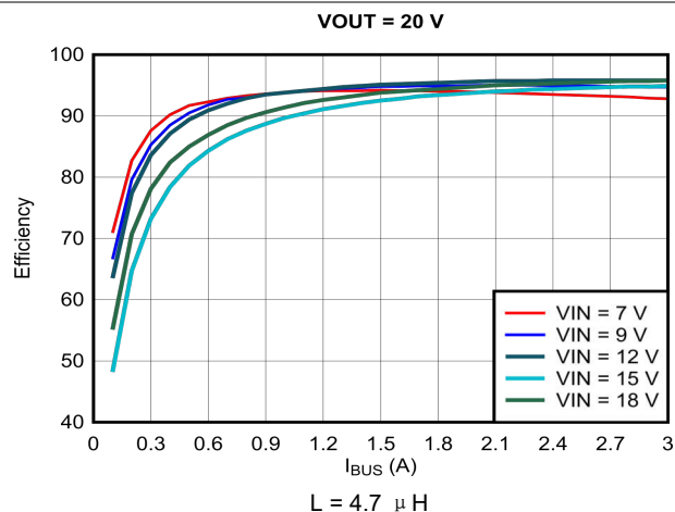
图 10-10. Efficiency vs Output Current ( I_{OUT} ), V_{OUT} = 20 V
