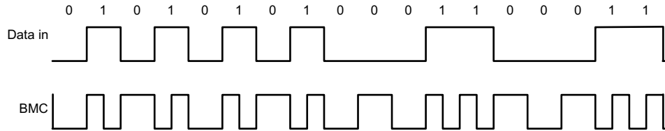
图 9-21. Biphasic Mark Coding Example
