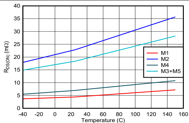
图 7-16. Buck-Boost Power FET R_{DS(ON)} vs Temperature
