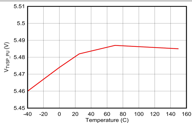
图 7-14. V_{TVSP\_PU} vs Temperature
