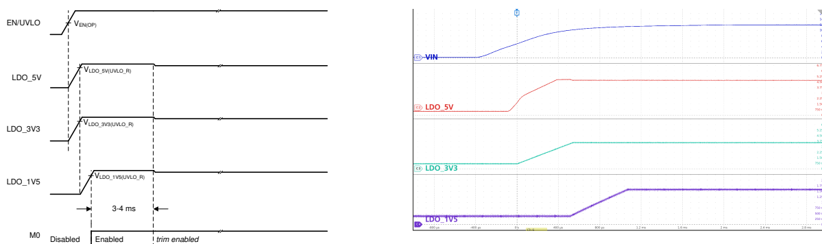
图 9-1. EN/UVLO and LDO Sequencing
