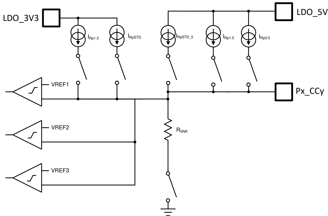
图 9-27. Plug and Orientation Detection Block
